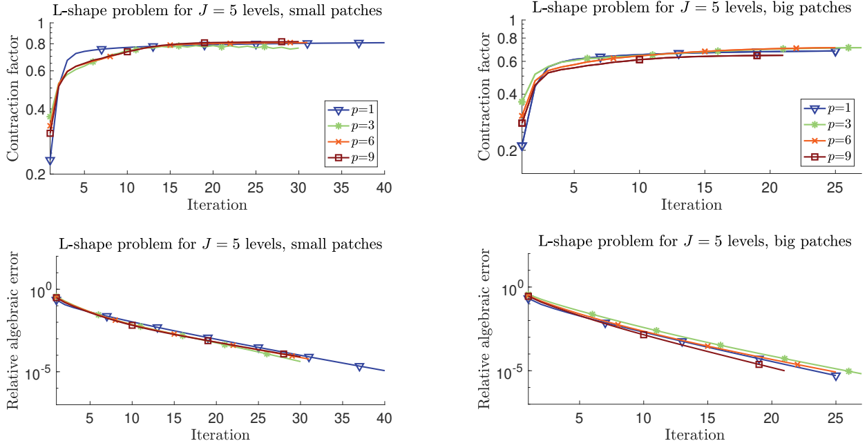
Figure 5: L-shape problem (6.3), w_1 = d + 1 , w_2 = J : results of the solver (4.6) for p' = p in (2.10a), “small” (left) and “large” (right) patches, and stopping criterion (6.4); top: error contraction factors \|\nabla(u_J - u_J^{i+1})\|/\|\nabla(u_J - u_J^i)\| ; bottom: relative algebraic error \|u_J - u_J^i\|/\|u_J\| .
