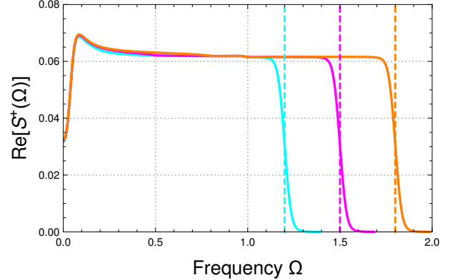
Figure 10. Emission noise S^+(\Omega) for a symmetric N-dot-S junction with \Gamma_N = 0.02 , at voltages V = 1.2\Delta, 1.5\Delta and 1.8\Delta (indicated by dashed vertical lines). Compare with Fig. 4 for the case of a NTS junction.
