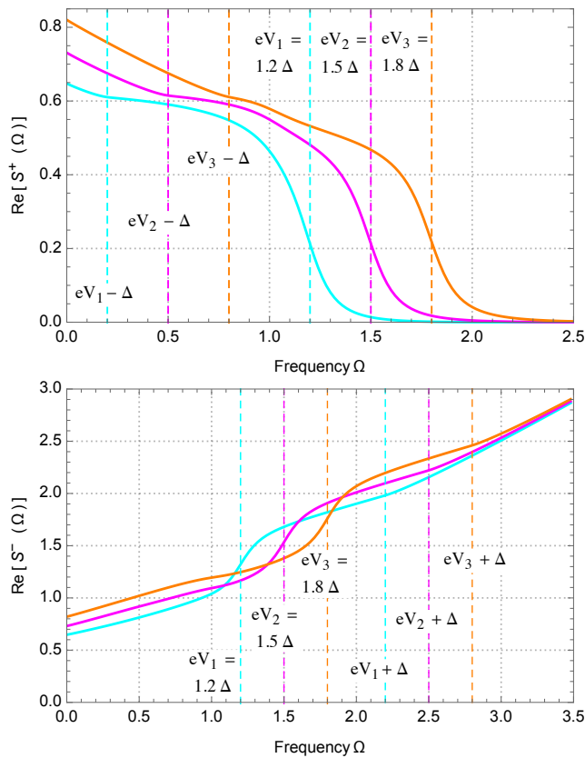
Figure 5. Emission noise S^+(\Omega) and absorption noise S^-(\Omega) (in units of e^2\Delta/h ) as a function of frequency \Omega (in units of \Delta ) at transparency \tau = 0.4 beyond the gap |eV| > \Delta , for three different values of the voltage bias ( eV = 1.2\Delta, 1.5\Delta and 1.8\Delta ).
