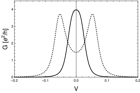
Figure 8. Differential conductance G = dI_N/dV , for the current to the normal lead I_N , in a N-dot-S junction, with symmetric couplings ( \Gamma_N = \Gamma_S = 0.02 , full line) and asymmetric couplings ( \Gamma_N = 0.02 , \Gamma_S = 3\Gamma_N , dotted line), as a function of the voltage of the normal lead. Other parameters : \epsilon = 0 , 1/(k_B T) = 300 . The superconducting gap \Delta is the unit of energy.
