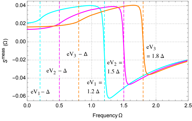
Figure 7. Measurable noise (in units of e^2 K \Delta / h ) as a function of frequency \Omega (in units of \Delta ) at low transparency ( \tau = 0.02 ) for an electron temperature T_e = 0.01\Delta and a detector temperature T_{LC} = \Delta .
