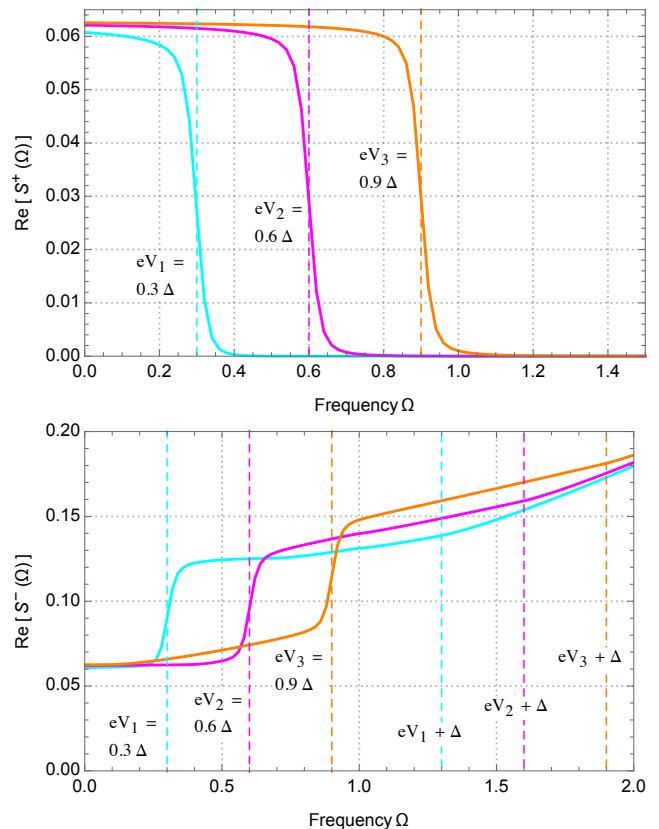
Figure 3. Emission noise S^+(\Omega) (top) and absorption noise S^-(\Omega) (bottom) as a function of frequency \Omega (in units of \Delta ) at low transparency ( \tau = 0.02 ) computed in the subgap regime |eV| < \Delta for three different values of the voltage bias ( eV = 0.3\Delta, 0.6\Delta and 0.9\Delta ), and expressed in units of e^2\Delta/h .
