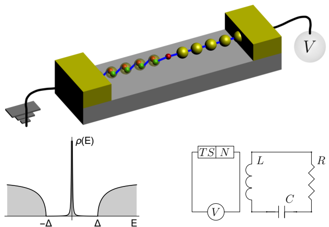
Figure 1. Top: schematic view of a junction between a normal metal (yellow dots) and a topological superconductor (red-green dots, with a red Majorana bound state at its end); the normal metal is biased at voltage V . Bottom left: topological superconductor density of states, with a central peak at zero energy due to the Majorana bound state, and square root behavior outside the gap. Bottom right: the principle of the noise detection, using the inductive coupling to a RLC circuit. 20
