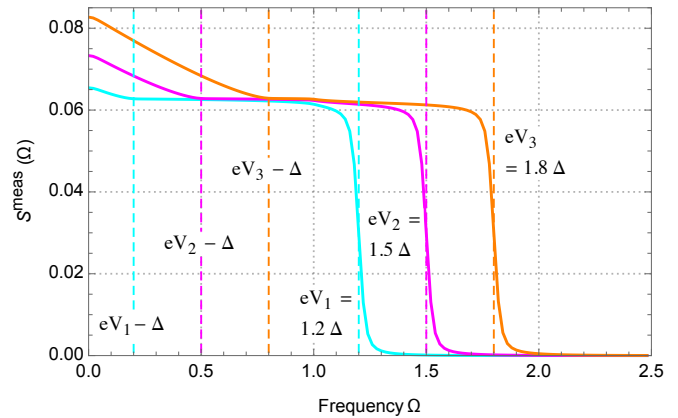
Figure 6. Measurable noise (in units of e^2K\Delta/h ) as a function of frequency \Omega (in units of \Delta ) at low transparency ( \tau = 0.02 ) for electron and detector temperatures T_e = T_{LC} = 0.01\Delta .
