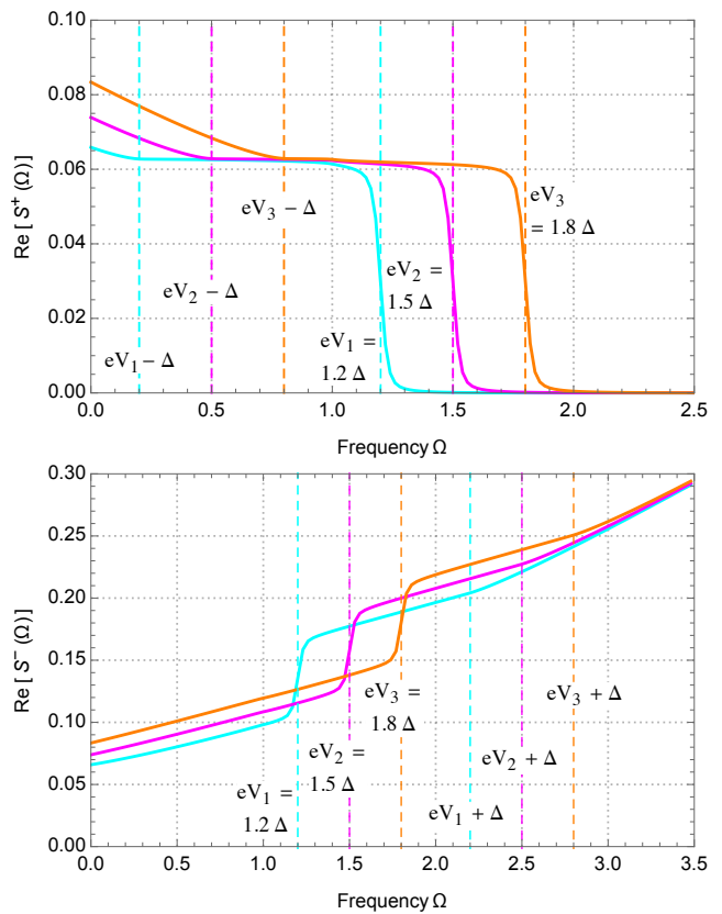
Figure 4. Emission noise S^+(\Omega) (top) and absorption noise S^-(\Omega) (bottom) as a function of frequency \Omega (in units of \Delta ) at low transparency ( \tau = 0.02 ) computed beyond the gap |eV| > \Delta for three different values of the voltage bias ( eV = 1.2\Delta, 1.5\Delta and 1.8\Delta ), and expressed in units of e^2\Delta/h .
