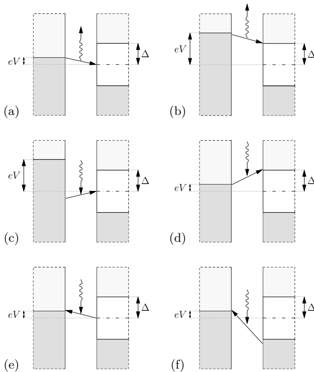
Figure 2. Energy diagram of a NTS junction. In medium grey are represented the occupied electronic states and in light grey the empty states. (a)-(b) emission processes, (b) is not available for a bias eV below the gap \Delta , (c)-(d) absorption processes involving a transition from the metal to the superconductor, (e)-(f) absorption processes with transitions to the metal. Straight lines correspond to the transfer of electrons while wiggly lines are associated with the absorption or emission of photons.
