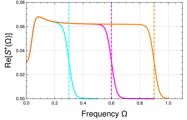
Figure 9. Emission noise S^+(\Omega) for a symmetric N-dot-S junction with \Gamma_N = 0.02 , at voltages V = 0.3\Delta, 0.6\Delta and 0.9\Delta (indicated by dashed vertical lines). Compare with Fig. 3 for the case of a NTS junction.
