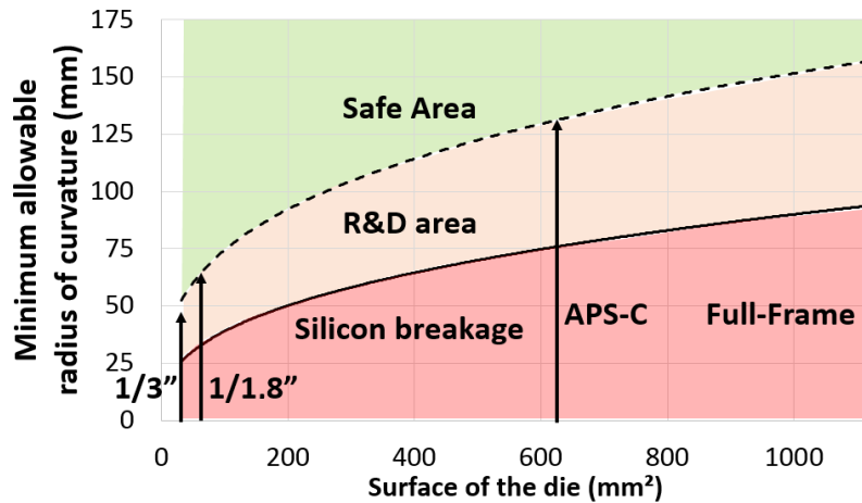
Fig. 1. Results of breakage limits considering two failure criteria, \sigma_{1,max1} = 200\text{MPa} and \sigma_{1,max2} = 500\text{MPa} , for 1/3" format, 1/1.8" format, APS-C format, Full frame format, at 100 microns of thickness.
