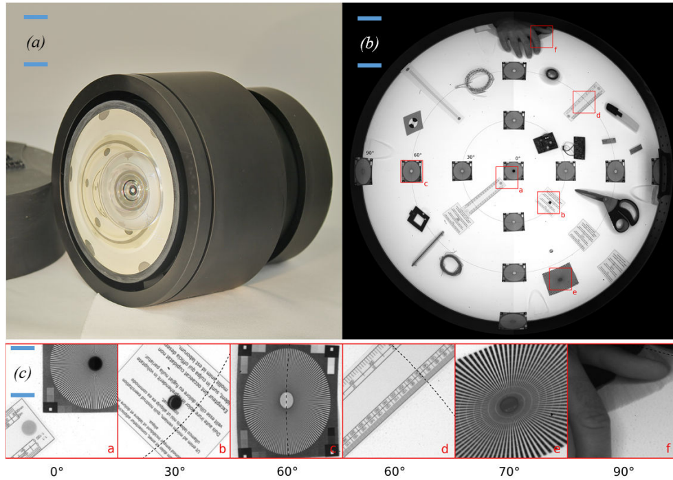
Fig. 5. a) Simplified zoom prototype; b) Image acquisition at 8 mm focal length F/4 of an object located at 400 mm from the objective in all directions; c) zoomed parts of image acquisition.
