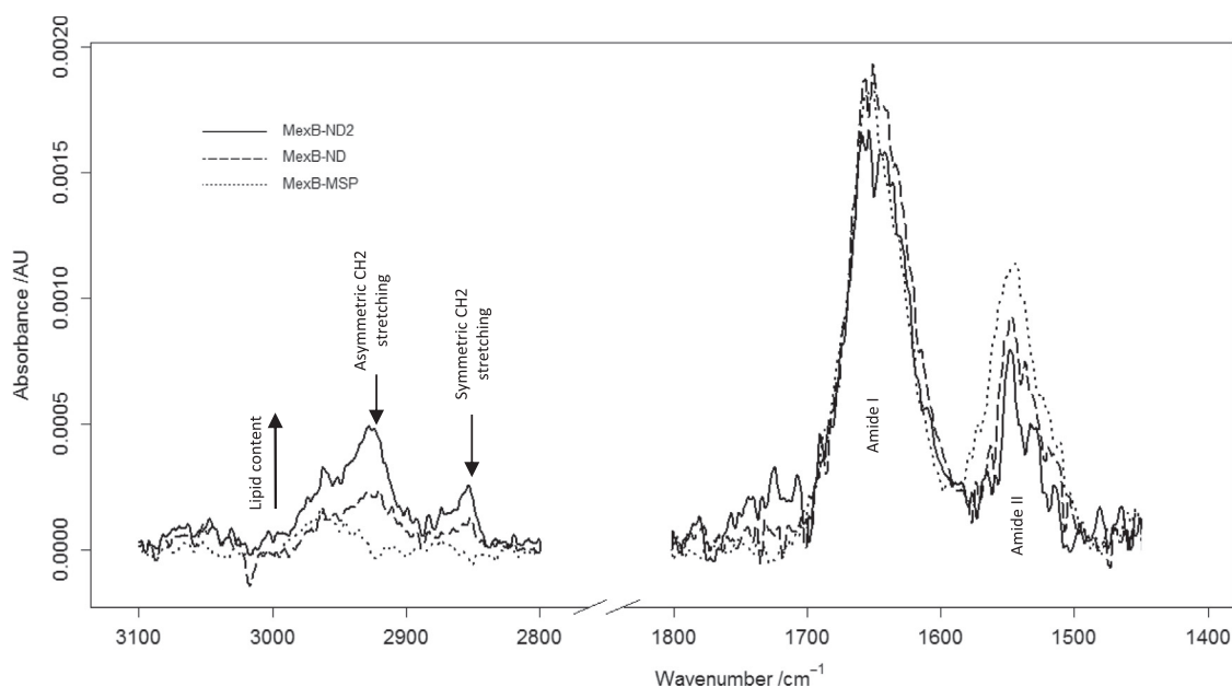
Fig. 5. ATR-FITR characterization of lipid content for MexB reconstituted in ND or with MSP alone.
