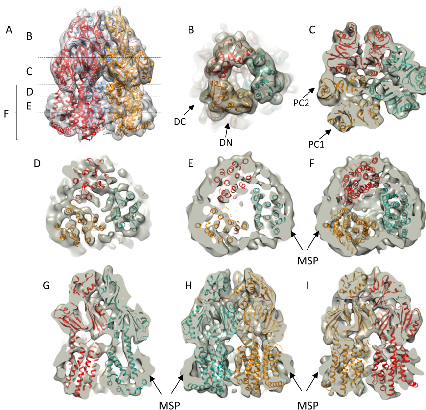
Fig. 3. Fitting of MexB crystal structure within the cryo-EM map.
