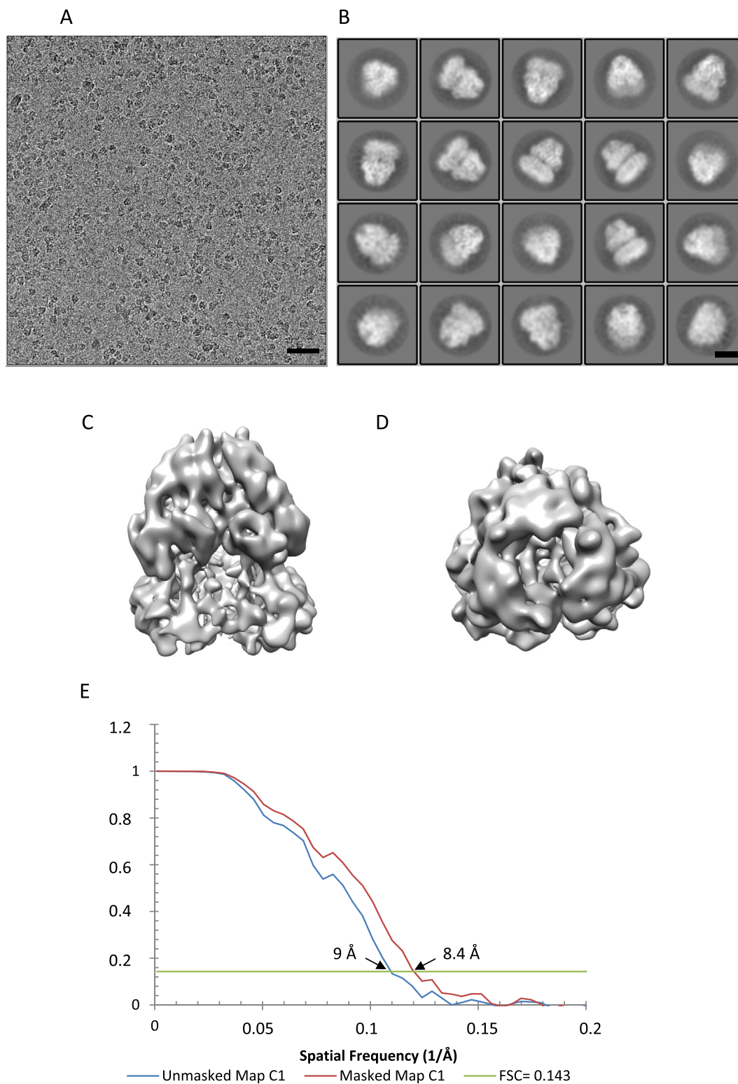
Fig. 2. Cryo-EM data and image processing of MexB-MSPE3D1. A) Representative cryo-EM micrograph. Scale bar 50 nm. B) Average images after 2D classification. Scale bar 7 nm. C–D) Side and top views of MexB-MSP cryo-EM reconstruction. E) Resolution curve.
