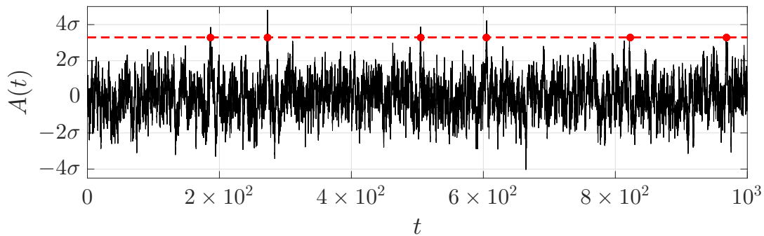
(a) Sample timeseries (black curve), generated from an Ornstein–Uhlenbeck process (22) ( \alpha = 1 , \epsilon = 1/2 ; \sigma = 1/\sqrt{2} is the standard deviation). We are interested in fluctuations which reach a prescribed threshold a (red curve). These events are identified by the red dots.
