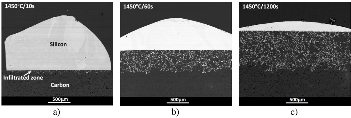
Figure 3. BSE images of the infiltrated zones at 1450°C produced in: a) 10 seconds, b) 60 seconds, and c) 1200 seconds.
