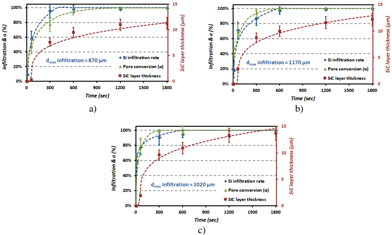
Figure 12. Experimental values (symbols) and calculated curves (dotted lines) of the kinetics of infiltration (%), pore conversion (%) and SiC layer thickness ( \mu\text{m} ) at: a) 1450^{\circ}\text{C} , b) 1500^{\circ}\text{C} , and c) 1550^{\circ}\text{C} .
