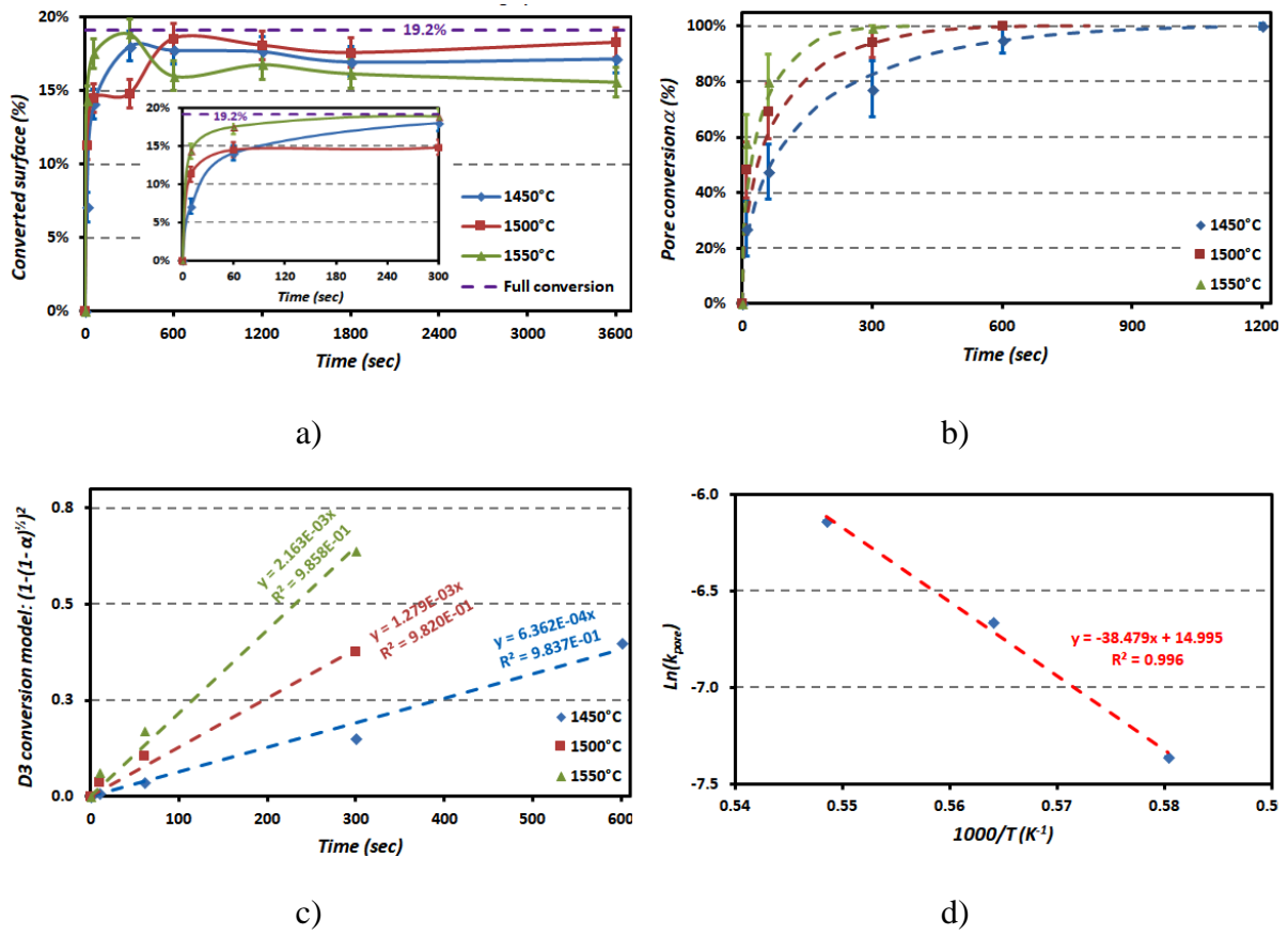
Figure 7. Reaction zone within the pores of the substrate: a) evolution of the overall conversion percentage of the infiltrated area (in insert, focus on short durations), b) evolution of pore conversion percentages and plots of the D3 laws, c) fit of the pores conversion ratios with D3 law, and d) Arrhenius plot of the role of pore conversion.
