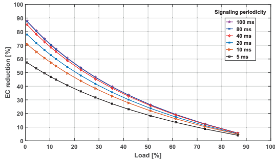
Fig. 6. Energy consumption reduction using ASMs depending on the signaling periodicity
