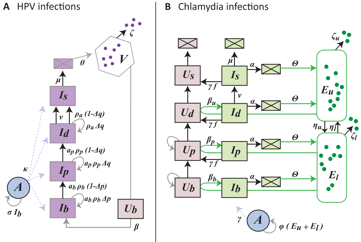
Fig 5. Flow diagram of the infection models for HPV (A) and chlamydia (B). HPV virions, V , only infect uninfected basal cells, U_b , to become basal infected cells, I_b . Since HPV is non-lytic, infected cells follow the typical epithelial life-cycle up to the surface passing through different life stages (parbasal I_p , differentiated I_d , differentiated at the surface I_s ). Model 3. In the case of C. trachomatis , the elementary bodies, EBs, start the infection by infecting uninfected cells in the upper layers ( \beta_u U_d E_u creates I_d ). The EB populations start in the upper layers, E_u , and then migrate down, \eta_u , into the lower layers, E_l . As EBs migrate down layers they enter uninfected cells ( U_b and U_p ) and create infected cells ( I_b and I_p ) which die at rate \alpha (boxes with square represent dead cells). The host immune response, A , is activated by infected basal cells in the case of HPV and all EBs in the case of C. trachomatis . Model 4. Note that for wart-associated HPV infections \rho_a = 0 and \alpha_b = \alpha_p = 1 . See Table 3 for parameter descriptions and estimates.
