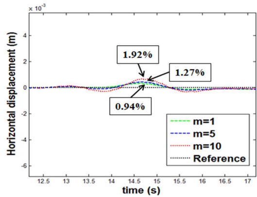
Fig.18 Horizontal displacements for Kosloff at the observation point using different time step ratios m
