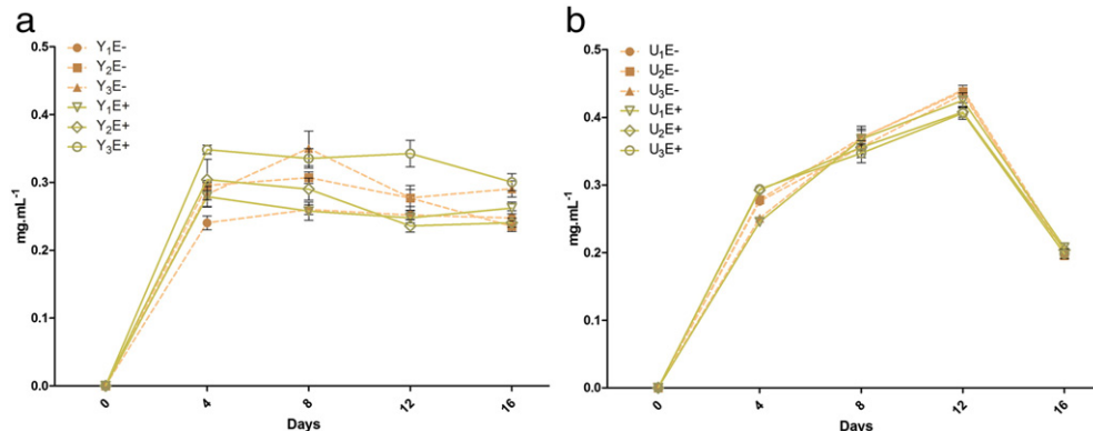
Fig. 5. Sugar content kinetics in the culture medium during 16 d of culture with (a) yeast extract, and (b) urea, as nitrogen source; and with 3 g/L (+) or 0 g/L (–) of ethanol. Bars indicate the mean of the data, and whiskers the standard error, n = 3 . The subscript numbers indicate concentration in g/L.
