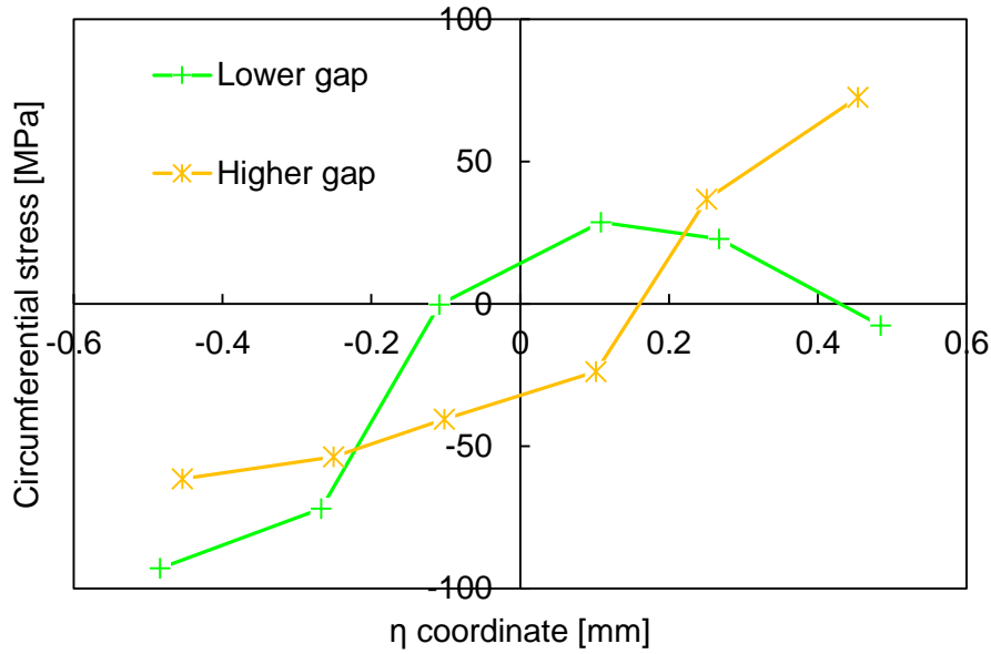
Figure 13. Difference between the circumferential stress distributions in the intact ring and in the split-ring, at the middle section of the Top ring.
