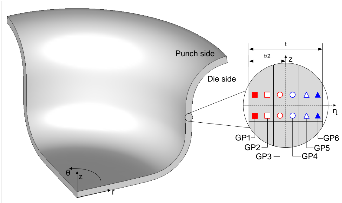
Figure 3. Positioning of the cylindrical coordinate system in the formed cup and of the local coordinate system \eta for the through-thickness stress analysis.
