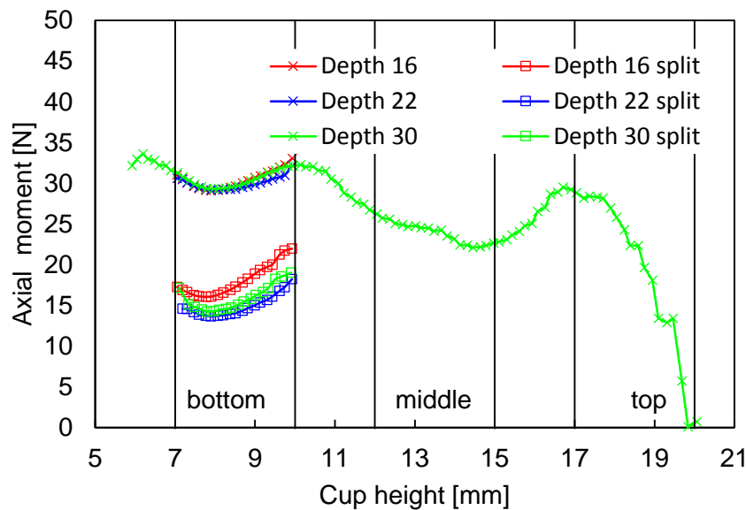
22 23 24 25 26 27 28 29 30 31 32 33 34 35 36 37 38 39 40 41 42 43 44 45 46 47 48 49 50 51 52 53 54 55 56 57 58 59 60 61 62 63 64 65 Figure 17. Axial moment (per unit length) distributions along the cup wall at the end of the cup forming and unloading stage and in the intact ring for the Lower gap, using different punch displacements.
