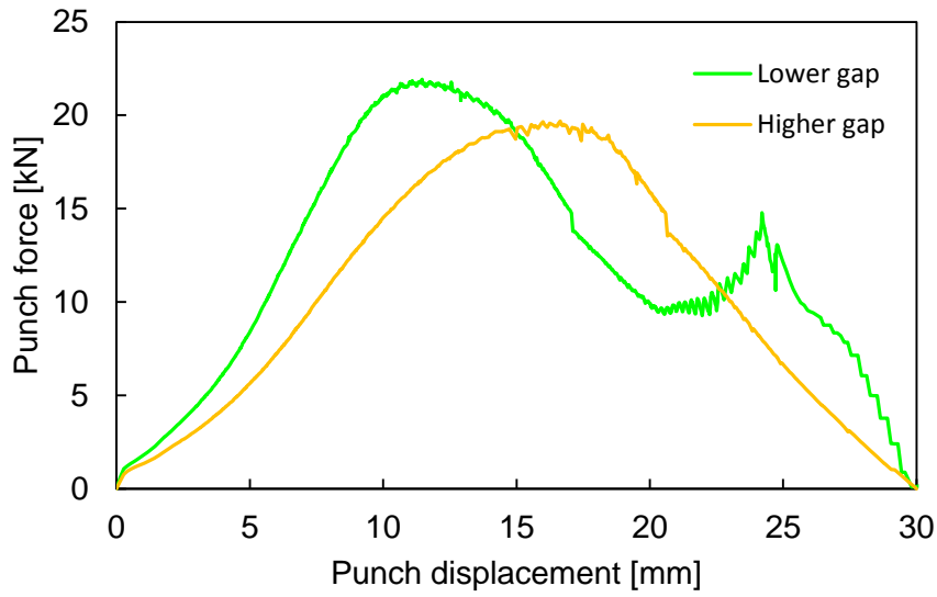
Figure 5. Numerical punch force evolution for the two different values of gap between the die and the punch.
