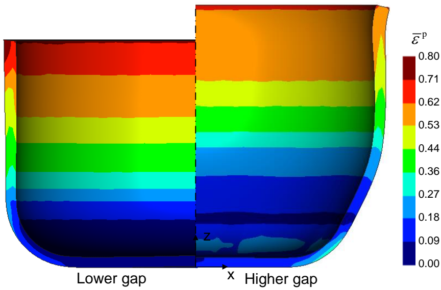
Figure 6. Equivalent plastic strain distribution plotted on the final shape of the cylindrical cups.
