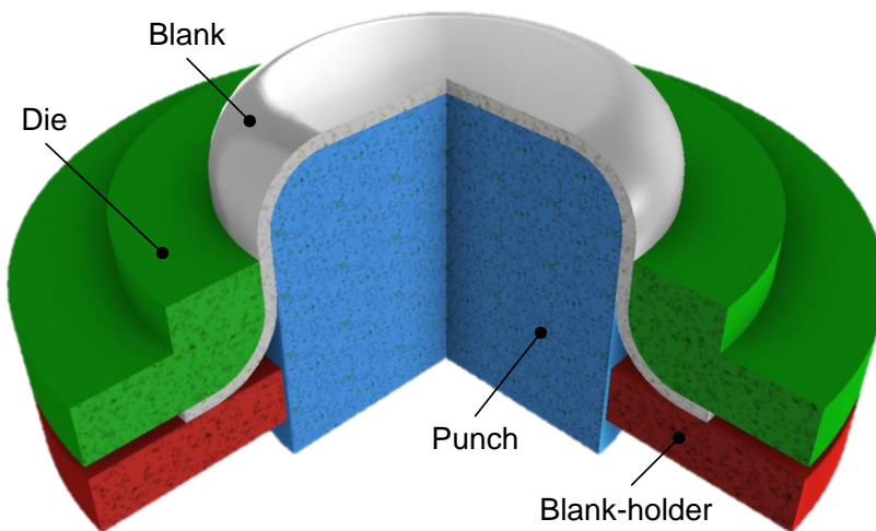
Figure 1. Schematic representation of the forming tools considering a gap between the punch and the die of 1.125 mm.
