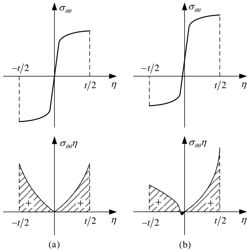
Figure 4. Schematic representation of the integrand for moment computation for: (a) a symmetric through-thickness stress distribution; (b) a non-symmetrical through-thickness stress distribution, for the circumferential stress, adapted from [24].
