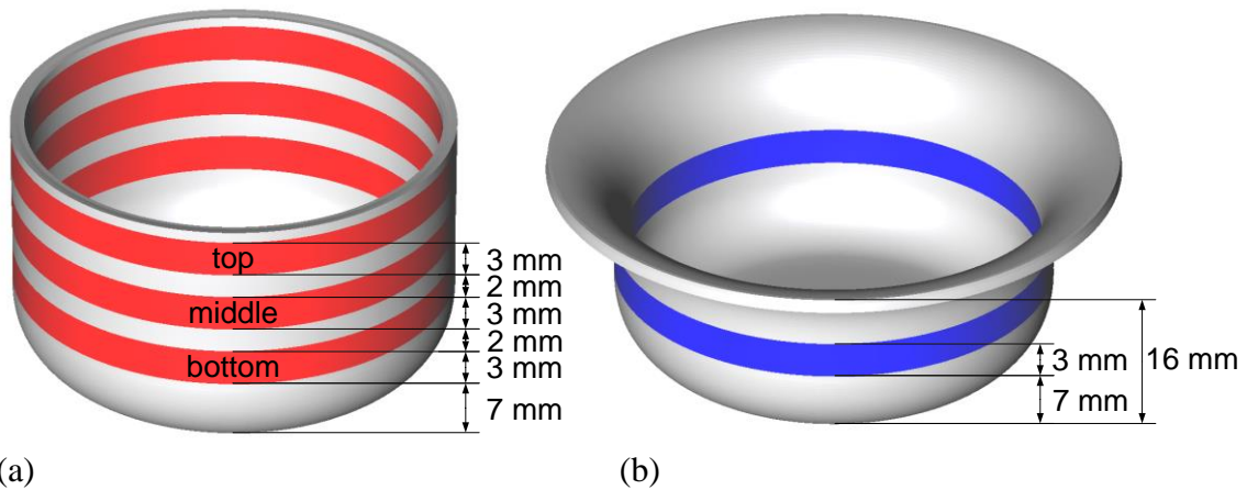
Figure 2. Positioning of the ring(s) in the cylindrical cup: (a) fully drawn cup; (b) for a fixed punch displacement of 16 mm.
