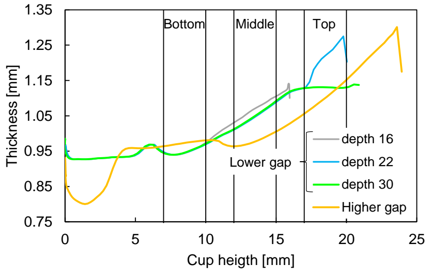
Figure 7. Thickness distribution along the cup height at the end of the cup forming and unloading stage, for the standard punch displacement of 30 mm, for both gap values, and for the punch displacement of 16 and 22 mm for the lower gap value.
