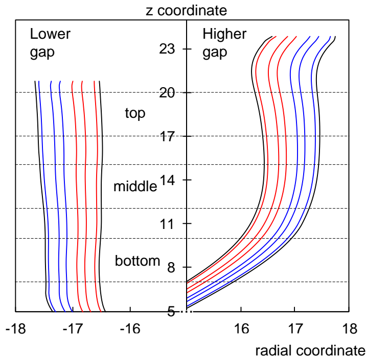
Figure 8. Section profile of the cup wall at the end of the forming and unloading stages, highlighting the relative position of the six through-thickness integration points.
