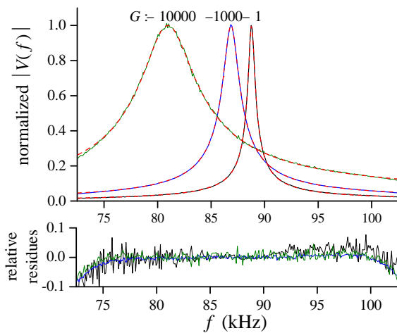
Figure 8: Examples of measured response signals with the direct coupling scheme (a) of Fig. 7 for G = -1 , -1000 , and -10000 . The PU coil pair described in Sec. 3.5 was connected in series ( L = 2.08 mH) and tuned close to 87.45 kHz. The fits by Eq. 14 (red dotted lines) yield Q' = 141.5 , 60.3, and 16.6, respectively, instead of Q = 157 for a weak coupling measurement (not shown). Relative residues (lower plot) do not exceed 7% in the fitting frequency range.
