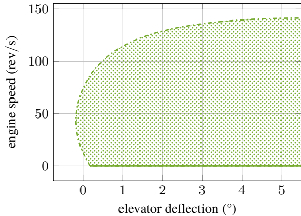
Figure 5: Stable inputs in the event of loss of elevator: engine speed n over surface position \eta_0 .
