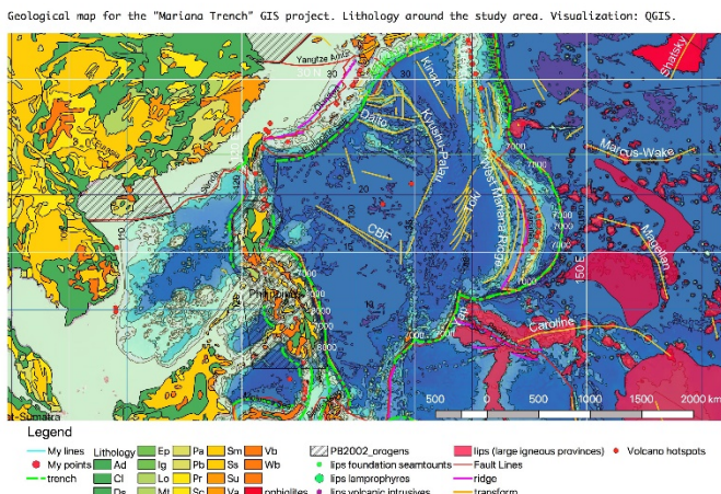
Figure 2. Lithology of the Mariana Trench area, Pacific Ocean (This map was created by QGIS software)
