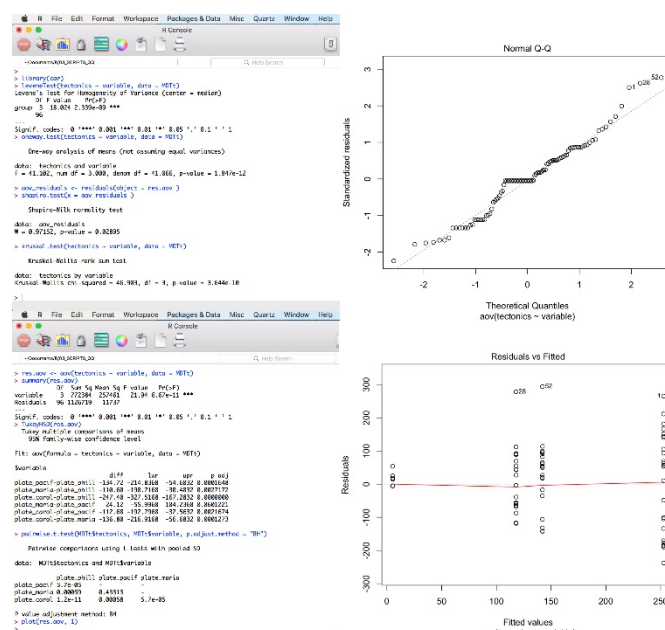
Figure 11. ANOVA hypothesis testing
