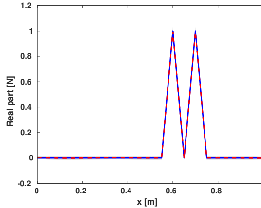
Figure 4: Complete Bayesian formulation – Real part of the reconstructed force vector – (—) Reference, (---) Median of the samples and (■) 95% credible interval
