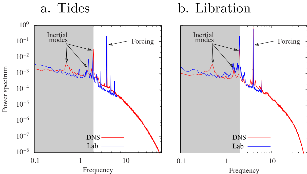
FIG. 4. Power-spectrum of the saturated turbulent flow in (a) tidal experimental and numerical studies and (b) libration experimental and numerical studies. In all cases, the forcing frequency is equal to four times the spin frequency. Ekman numbers are respectively equal to E_{exp,tide} = 1.5 \times 10^{-5} , E_{num,tide} = 5 \times 10^{-5} , E_{exp,lib} = 2.7 \times 10^{-5} , E_{num,lib} = 10^{-4} . Reproduced from [34].
