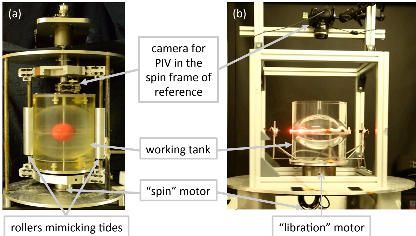
FIG. 2. Pictures of (a) the tides set-up at IRPHE, France and (b) the libration set-up at UCLA, USA (©A. Grannan). Typical radius of both tanks is 10cm, typical spin velocity is 30 – 180rpm.
