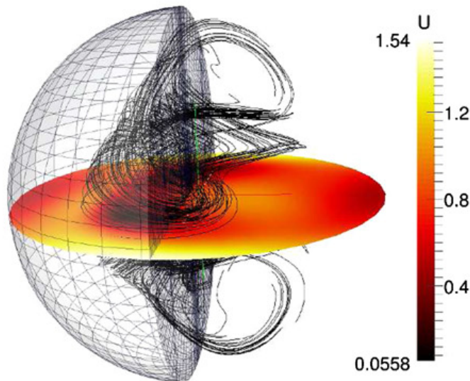
FIG. 5. Magnetic field lines and velocity magnitude in an equatorial slice in the tidal dynamo of Cébron and Hollerbach [38]. Here the Ekman number is E = 5 \times 10^{-3} and the magnetic Prandtl number (i.e. the ratio of viscosity and magnetic diffusivity) is Pm = 5 . Reproduced with permission from [38] (©AAS).
