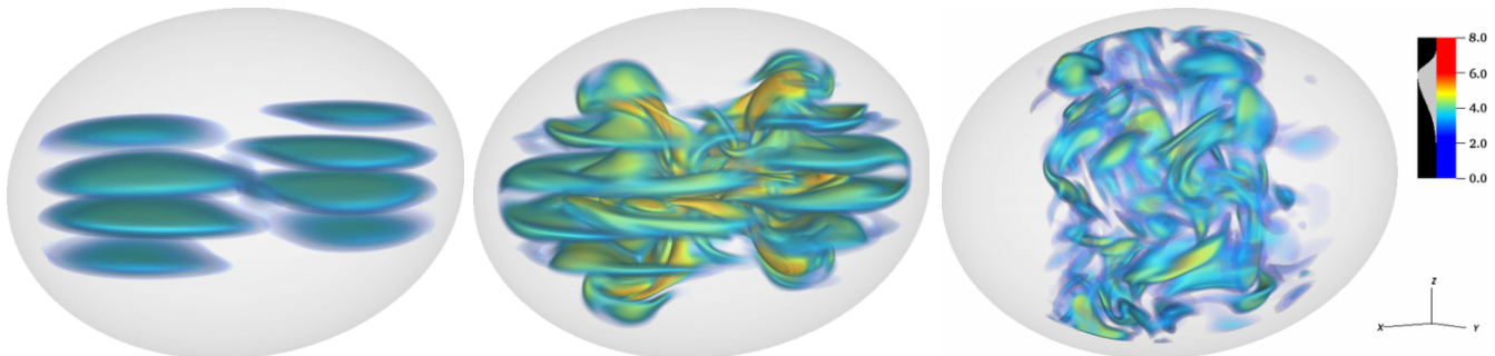
FIG. 3. Volume rendering of the enstrophy in the bulk of a librating ellipsoid, unstable to the libration driven elliptical instability. From left to right: inertial modes excited during the initial exponential growth of the instability; first saturation of the flow; and quasi-steady saturated turbulent state. For this numerical simulation, the libration frequency is equal to four times the spin frequency and the Ekman number E_{num,lib} = 10^{-4} . Reprinted from [36] with the permission of AIP Publishing.
