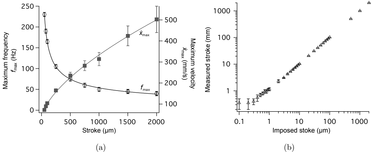
Figure 2: CHRONOS tribometer operating limits: a - maximum frequency and velocity as a function of set stroke; b - measured stroke as a function of the imposed stroke.
