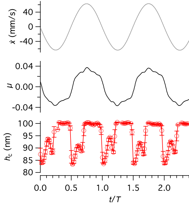
Figure 10: Superimposition of the velocity \dot{x} , the friction coefficient \mu and the central lubricant film thickness h_c measured at an oscillation frequency of 20 Hz.
