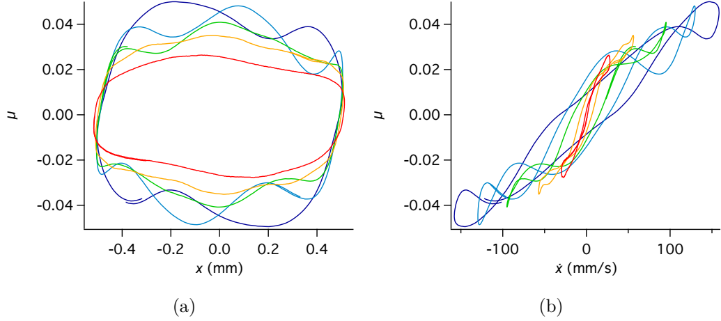
Figure 6: Friction instantaneous cycles at 48, 39, 27,16 and 7 Hz from purple-blue to red: a- as a function of the displacement x ; b - as a function of the velocity \dot{x} .
