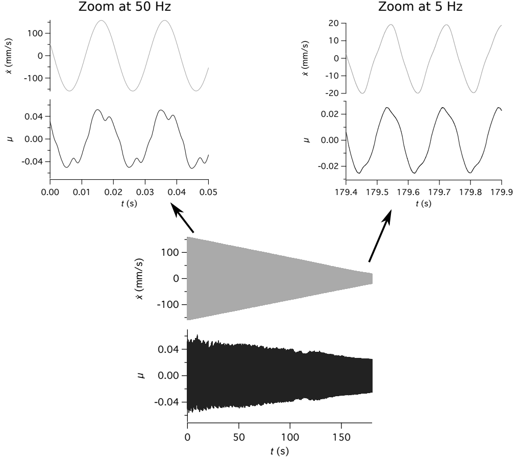
Figure 3: Velocity and friction coefficient synchronized temporal signals from 50 Hz to 5 Hz.
