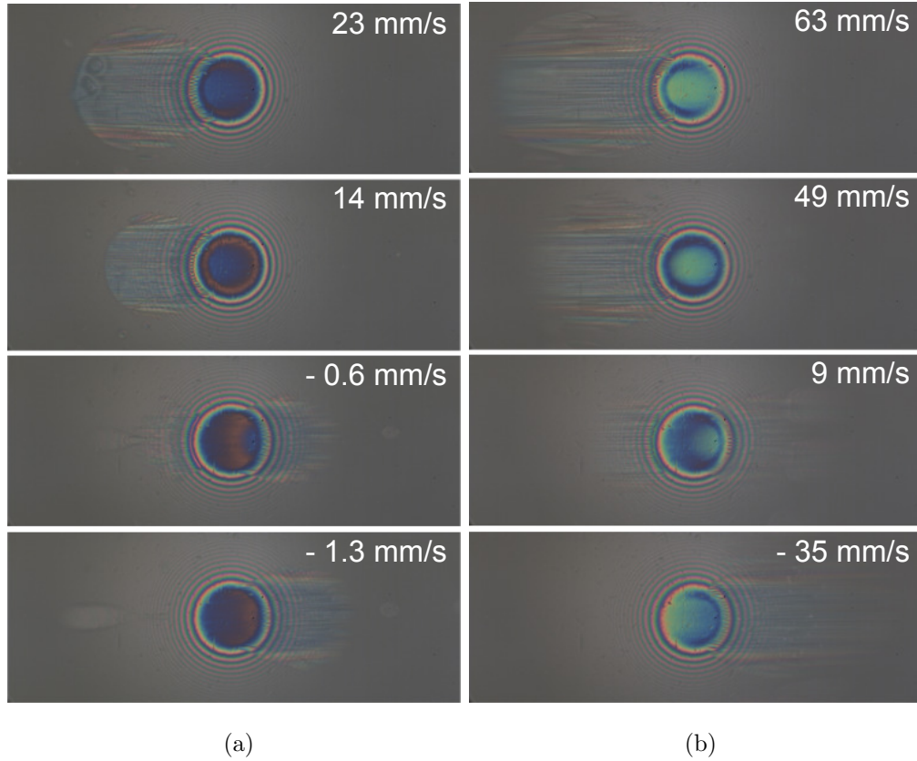
Figure 8: Interferometric images of the lubricated sliding contact (radius of 86\ \mu\text{m} ) extracted from videos with a frame rate of 180 fps (the velocity is positive for the lubricant flow direction from the right to the left): a- sliding frequency of 6 Hz; b- sliding frequency of 20 Hz.
