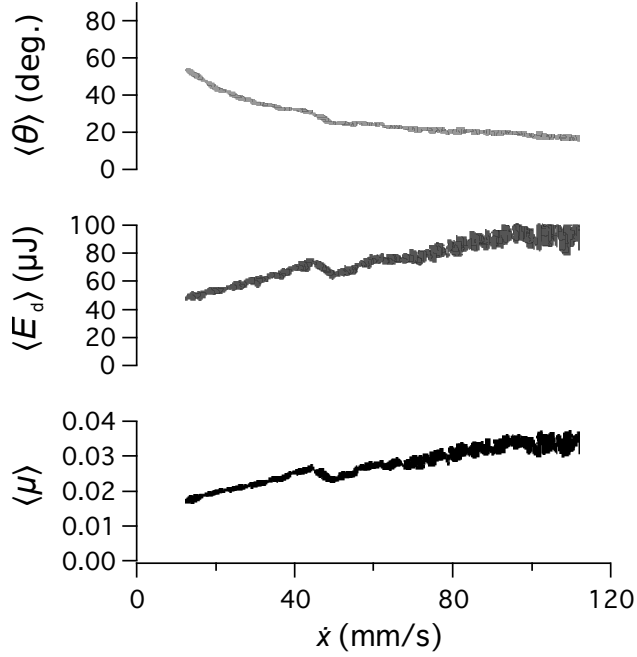
Figure 7: Averaged parameters of the sliding contact as a function of the velocity moving average (friction-velocity cycles tilt angle and average signals of dissipated energy and friction coefficient).
