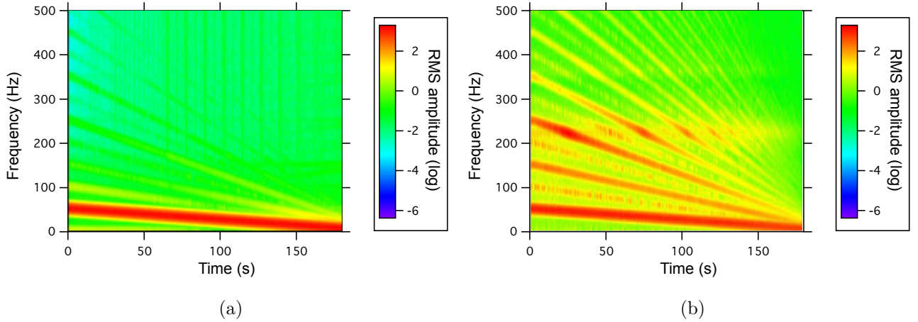
Figure 4: Time-frequency analysis: a - Displacement spectrogram; b - Friction coefficient spectrogram.
