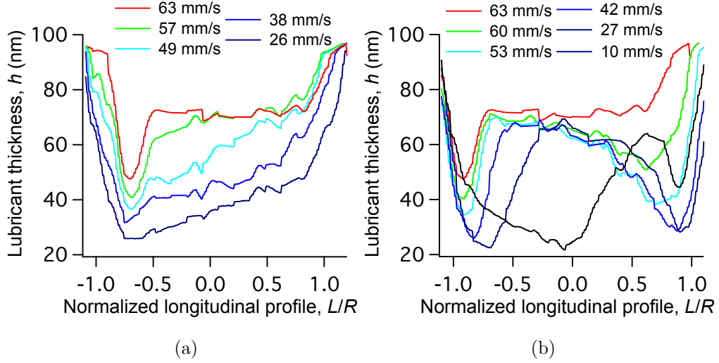
Figure 9: Lubricant film thickness longitudinal profiles over one stroke measured at an oscillation frequency of 20 Hz (with L/R the ratio between the longitudinal distance on the contact radius): a- during an acceleration from 0 to 62 mm/s; b- during a deceleration from 62 mm/s to 0.
