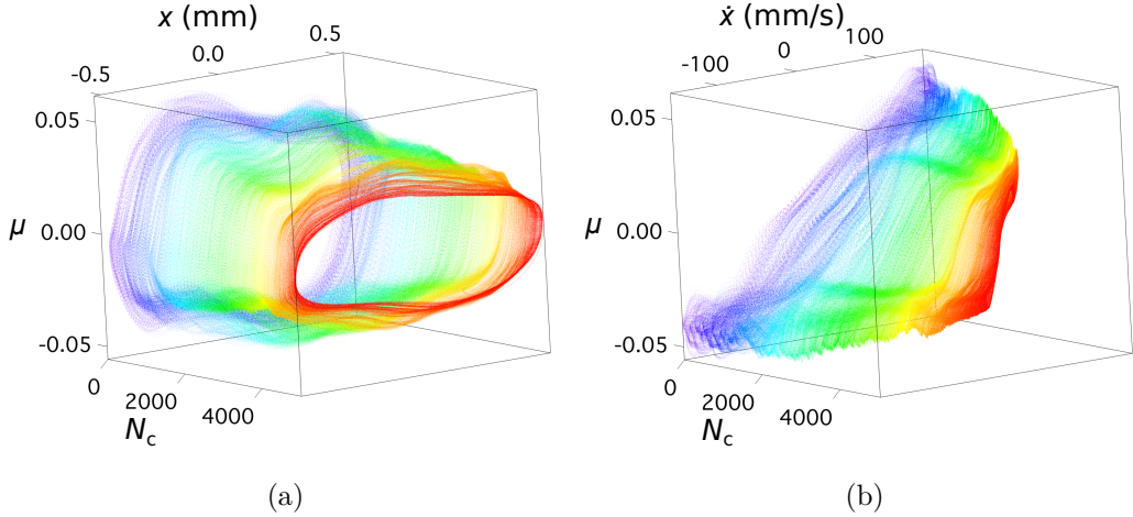
Figure 5: Log representations of friction considering the number of cycles N_c (rainbow color from purple-blue at 50 Hz to red at 5 Hz): a- as a function of the displacement x ; b- as a function of the velocity \dot{x} .
