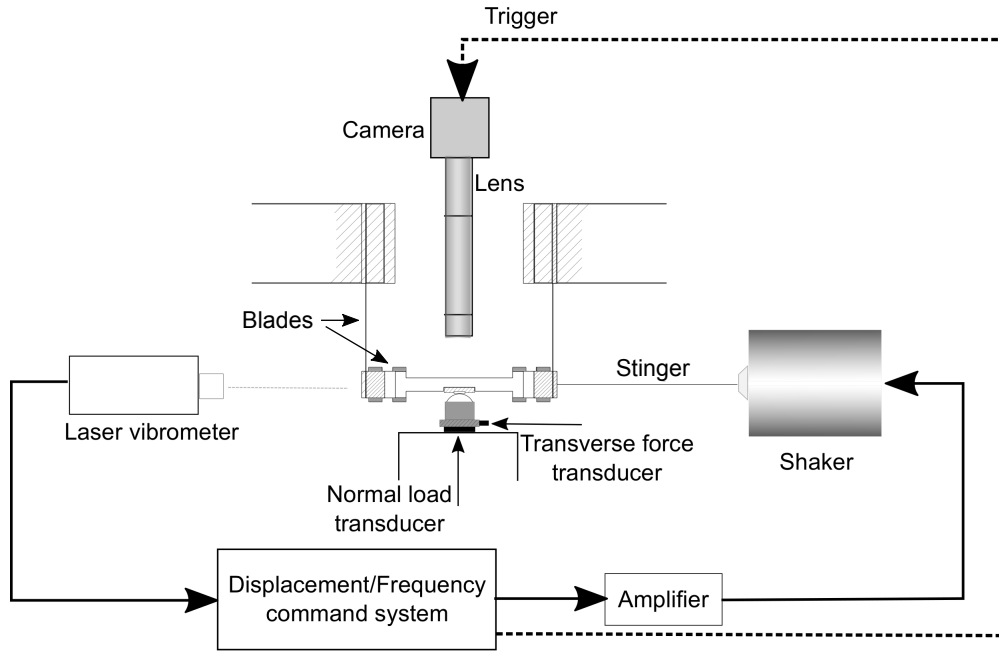
Figure 1: Instrumented forced oscillations tribometer (CHRONOS).
