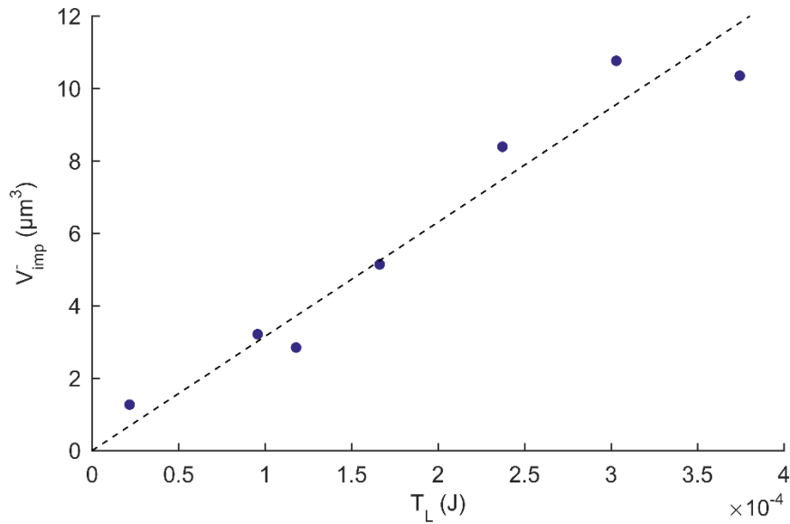
Fig. 12. Wear volume per impact versus energy loss at constant incidence angle equal to 30^\circ ; dotted black line: linear fit.
