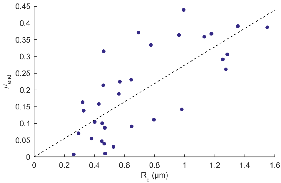
Fig. 10. Impulse ratio at the end of the wear test versus R_q roughness parameter of the wear scar; dotted black line: linear fit.
