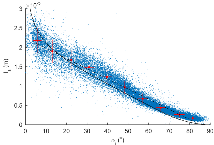
Fig. 5. Sliding distance versus incidence angle \alpha_i during impacts in water environment. Cloud: experimental data; solid line computed from Eq. (26); dotted line: linear fit of the experimental values.
