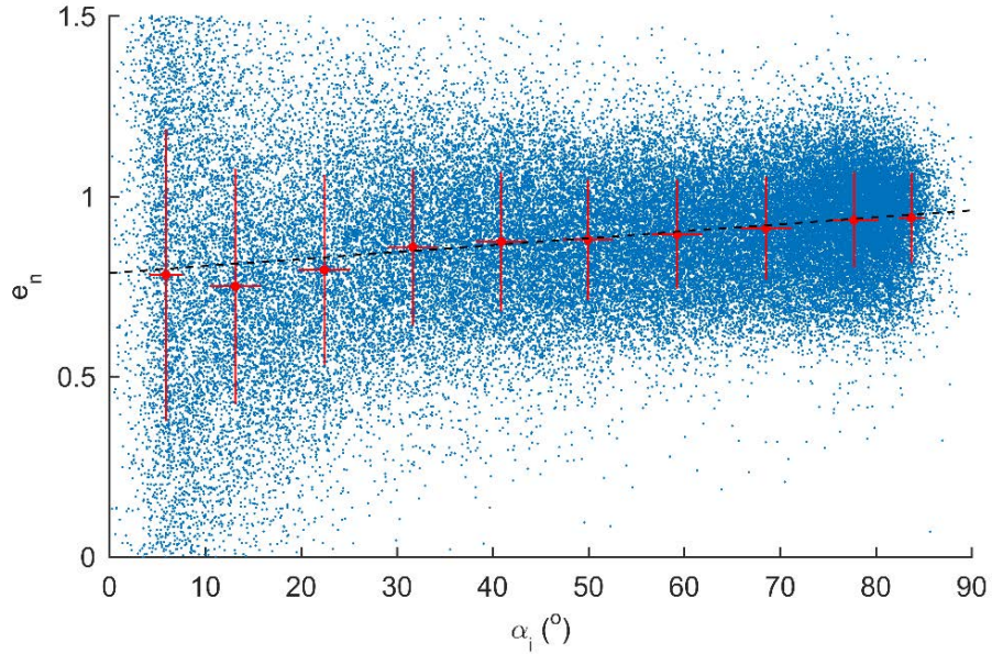
Fig. 2. Restitution coefficient vs incidence angle during impacts in water environment. Cloud: experimental data; broken black curve: linear fit.
