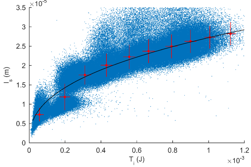
Fig. 6. Sliding distance versus incidence energy T_i during impacts in water environment at constant incidence angle equal to 30^\circ . Cloud: experimental data; solid black line computed from Eq. (26).
