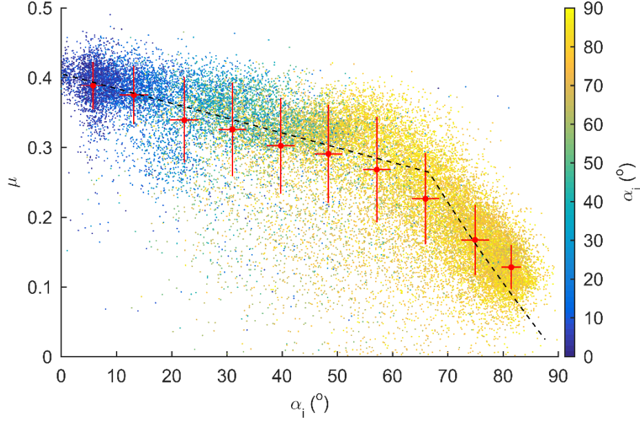
Fig. 3. Impulse ratio vs incidence angle during impacts in water environment. Cloud: experimental data; black curve computed from Eq. (16).
