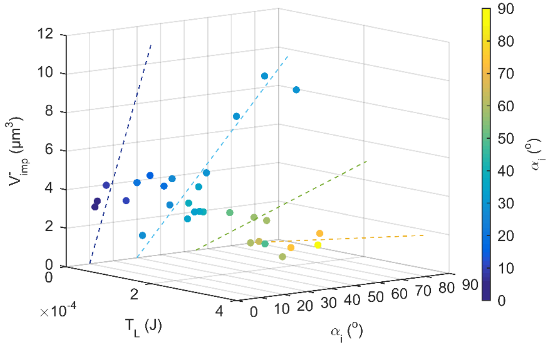
Fig. 13. Wear volume per impact versus impact energy loss and incidence angle; color: incidence angle; dotted lines: linear fits.
