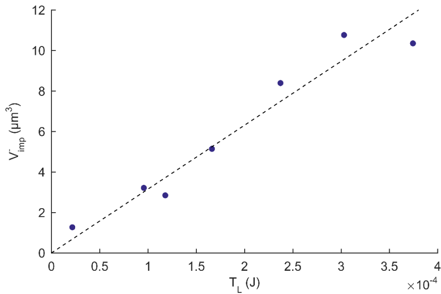
Fig. 12. Wear volume per impact versus energy loss at constant incidence angle equal to 30°; dotted black line: linear fit.
