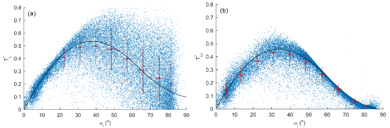
Fig. 4. (a) Total dimensionless energy loss T_L^* versus incidence angle \alpha_i during impacts in water environment. (b) Tangential dimensionless energy loss T_{Lt}^* versus incidence angle \alpha_i during impacts in water environment. Cloud: experimental data; solid black line respectively computed from Eq. (17) and Eq. (18).
