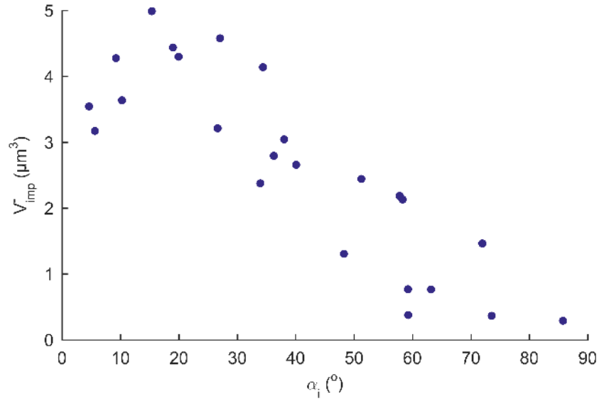
Fig. 11. Wear volume per impact versus incidence angle.
