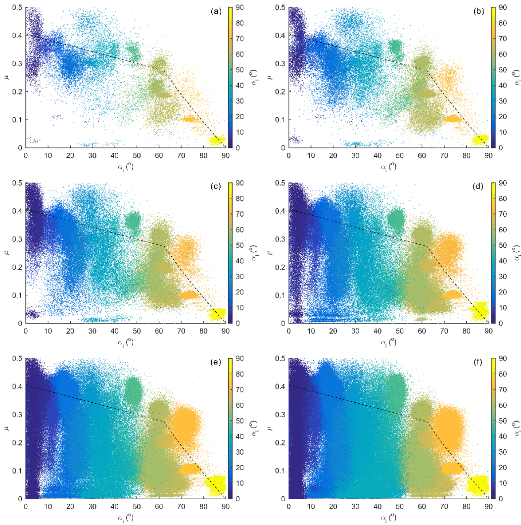
Fig. 7. Impulse ratio \mu versus incidence angle \alpha_i during long tests wear in water environment. Cloud: experimental data; black line computed from Eq. (16). (a) t=0-30 min. (b) t=0-1h . (c) t=0-2h . (d) t=0-4h . (e) t=0-8h . (f) t=0-16 h.
