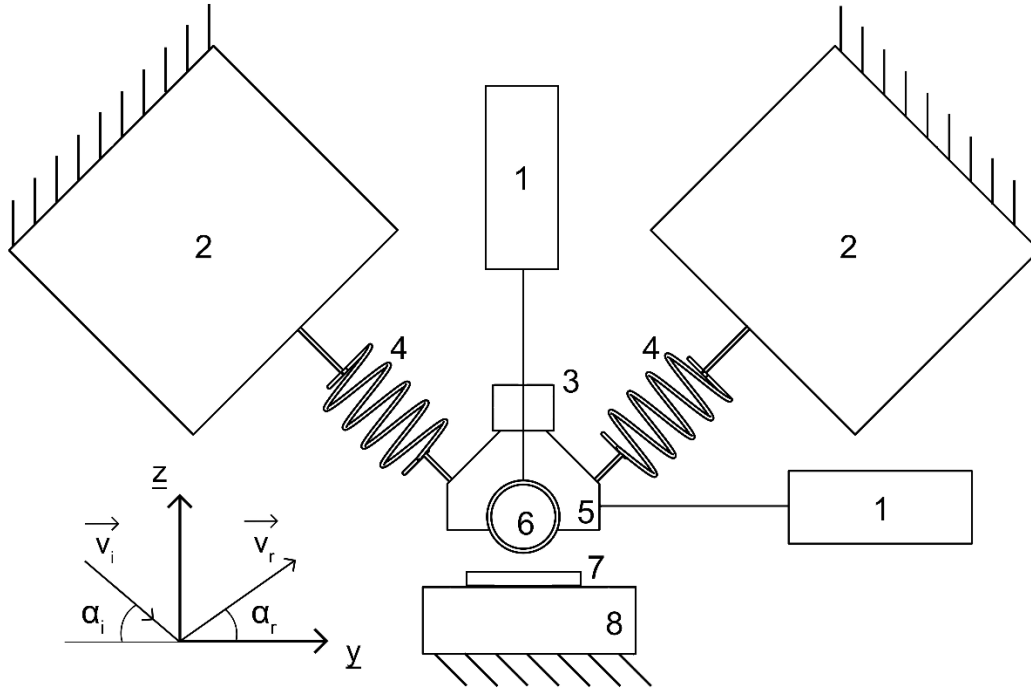
Fig. 1. Diagram of the impact wear test machine (1: Displacement sensors, 2: Shakers, 3: Loading mass, 4: Springs, 5: Tube holder, 6: SG Tube, 7: AVB holder and AVB sample, 8: Force transducer)
