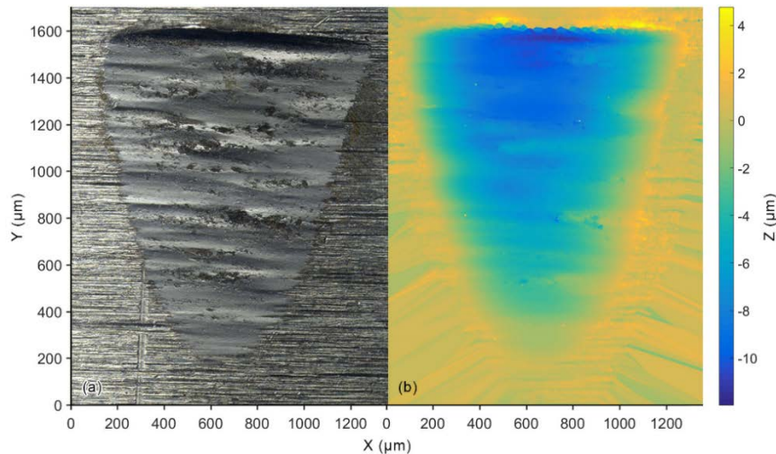
Fig. 8. Complete tube wear scar images. (a) SEM image. (b) Interferometry image.
