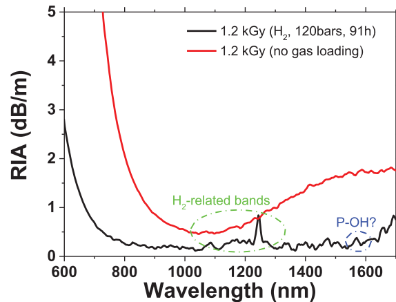
Fig. 9. Spectral dependences of the RIA measured after 1.2kGy \gamma -ray irradiation in the P-codoped multimode optical fiber and after exposure to \text{H}_2 loading (120 bars, 91 h, RT).
