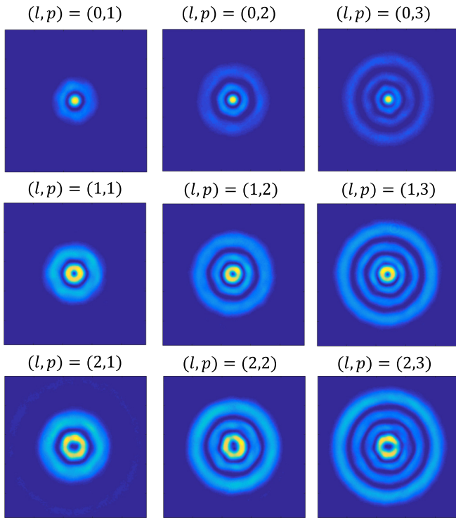
FIG. 6. Far-field intensity patterns reflected off the Bragg-Berry optical elements for l = (0, 1, 2) and p = (1, 2, 3) . Here the light source is a supercontinuum laser spectrally filtered at 532 nm with a 10-nm bandwidth.
