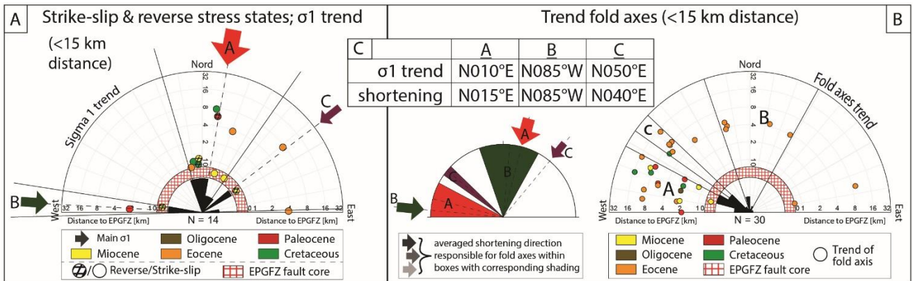
Fig. 16a: Plot showing trend of sigma 1 axes vs distance to the trace of the EPGFZ for measurements within 15 km of this fault. Arrows indicate dominant trends. Measurements obtained from the fault core are within the red hashed zone. Fig. 16b: Same principle as figure 16a but for fold axes derived from outcrops. Fig. 16c: Comparison between groups A, B and C from averaged \sigma_1 trend and averaged axes of contraction.
