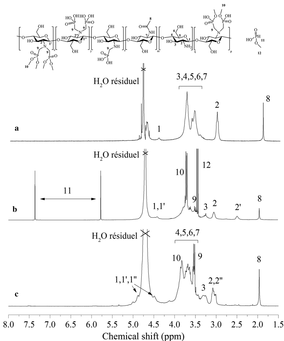
Fig. 3: 1 H NMR spectra recorded in D 2 O at 25 °C of: (a) N-chitosan 30, (b) P-chitosan 30 and (c) P-chitosan 30 after the hydrolysis at pH=1.
