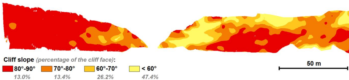
Figure 8: Classification of the cliff slope.
