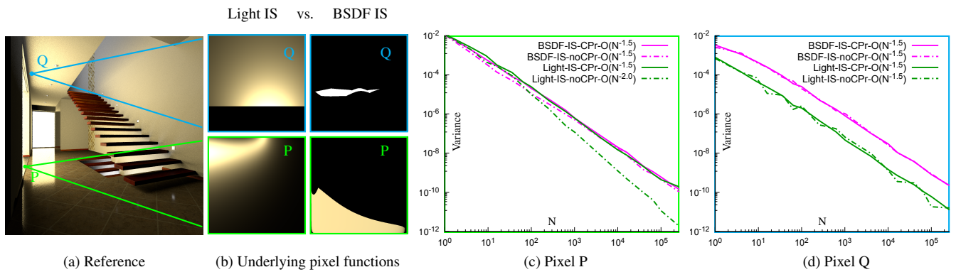
Figure 19: The convergence rate of MC integration with correlated (jittered) samples depends on the importance function (light vs. BSGF). We analyze two Pixels P & Q directly illuminated by a square area light source in (a). Pixel P is fully visible from the light source, which results in a smooth integrand when performing light source surface area sampling (visualized in bottom-left b) and a convergence rate of \mathcal{O}(N^{-2}) (c: dot-dashed green curve, all plots are in log-log scale). C_0 discontinuities in the integrand result in \mathcal{O}(N^{-1.5}) convergence, which can happen: when using homogenization or Cranley-Patterson rotation (CPr; solid green curve, more details in [SSC*19]); when the light source is partially occluded (Pixel Q); or when sampling the BSGF (in magenta) since this treats the boundary of the light as a C_0 discontinuity even when the light is fully visible (visualized in the second column of b). Figure reproduced from [SSC*19].
