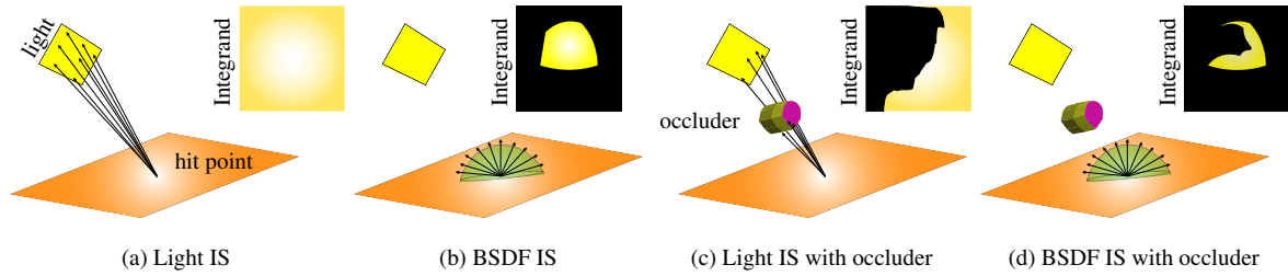
Figure 18: We illustrate the integrands (top-right in each column) for a shade point directly illuminated by an area light source for light IS and BSGF IS. (a) Light IS has a smooth underlying integrand when the light source is fully visible, unlike BSGF sampling (b), which sees light boundary as a C_0 discontinuity. Partially occluded shade points, on the other hand, always have a C_0 discontinuity (c,d). Figure reproduced from [SSC*19].
