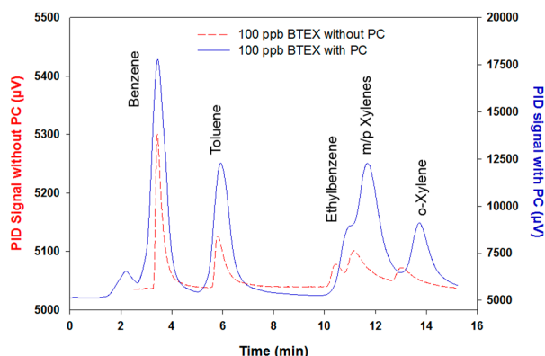
Figure 8. Red dashed line: Chromatogram of 100 ppb BTEX without preconcentration step (sample volume of 200 \mu\text{L} ). Blue solid line: Chromatogram of 100 ppb BTEX with preconcentration step (sample volume of 20 mL).
