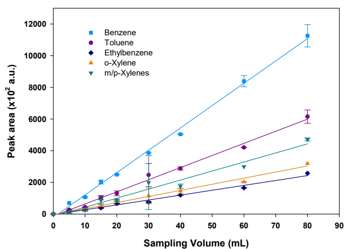
Figure 6. Peak area variation with sampling volume (BTEX concentration of 100 ppb). The vertical error bars show the standard deviation for duplicate injections.
