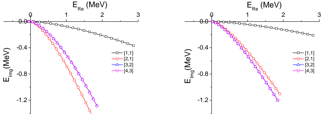
Figure 3: Resonance trajectories for J^\pi=1/2^+ state of {}^5\text{H} relative to {}^3\text{H} threshold. Each trajectory is made by 20 equidistant values of the V_5 strength parameter \lambda in eq. (5), starting from nearly threshold energy. The endpoint ( \lambda = 0 ) indicates the extrapolated physical values of the resonance predicted by the NN interaction. Left and right panels correspond to different parameterizations of V_5 ( \rho_0^2=78.4 \text{ fm}^2 and \rho_0^2=108.9 \text{ fm}^2 respectively, both with p = 0 ). The convergence of the results with respect to order of Padé approximant [m,n] are distinguished by colored curves.
