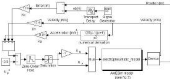
Fig. 6 Control feedback loop design with Simulink block diagram for a cosimulation protocol.
