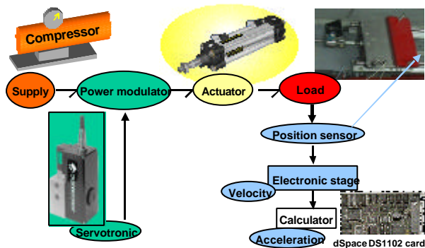
Fig. 3 Principe and example of an electropneumatic system.
