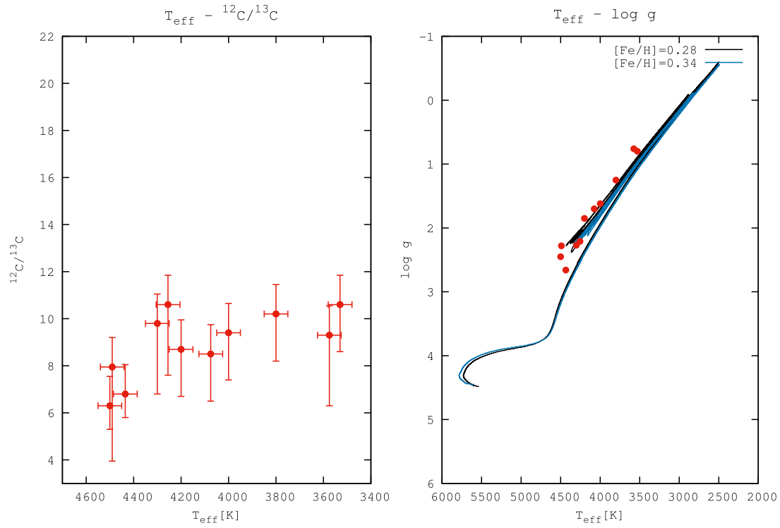
Figure 2. Left-hand panel: {}^{12}\text{C}/{}^{13}\text{C} ratio as a function of effective temperature from this paper. Right-hand panel: \log g as a function of effective temperature with evolutionary tracks from Lagarde et al. (2017) at different metallicities.
