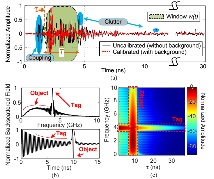
Fig. 2. (a) Scheme of the time-domain response for a frequency-coded chipless RFID tag. (b) Frequency and time signals and corresponding (c) STFT spectrogram representation of a theoretical 4 GHz resonator and a non-resonant object, both with the same amplitude.
