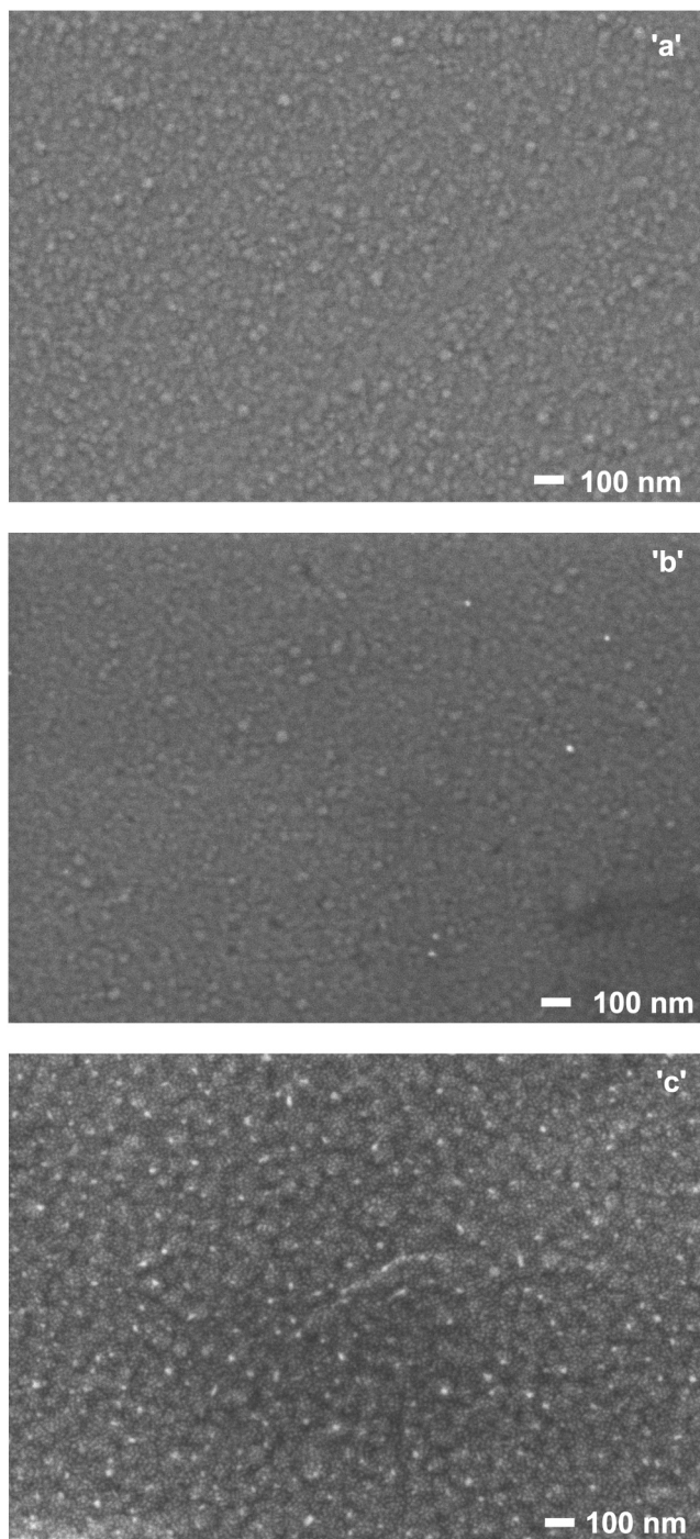
Fig. 1. SEM images of Si- \text{HfO}_2 :Er films: as-grown (a) and after annealing at 950 \text{ }^\circ\text{C} (b) and 1100 \text{ }^\circ\text{C} (c).
