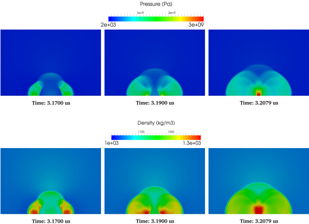
Figure 5: Pressure (top) and density (bottom) contour for a 2D bubble collapse showing the interaction of shock waves after the collapse of the bubble torus, corresponding to the second pressure peak of 3920 MPa at t = 3.2079 \mu s
