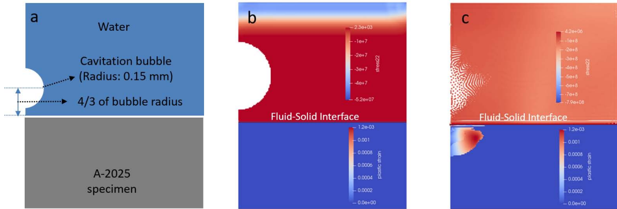
Figure 7. Fluid-structure interaction simulation of a bubble collapsing over a solid specimen: (a) Shows the computational domain for the simulation of a bubble of radius 0.15 mm with the center of the bubble at a distance of 4/3 times the radius from the interface, (b) SPH simulation where a pressure wave is generated from the top of the domain using repulsive particles producing a 50 MPa pressure wave approaching the bubble, (c) plastic strain developed in the material after the bubble collapse (contours in figure 7 (b) & (c) are for pressure in the fluid and plastic strain in the solid)
