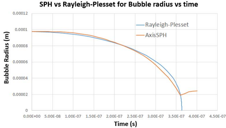
Figure 2. Comparison of bubble radius vs. time, SPH against Rayleigh-Plesset solution for a bubble collapse simulation (domain shown in figure 1)
