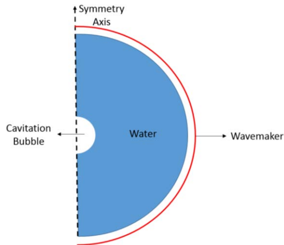
Figure 1. Simulation domain for bubble collapse simulation in 2D axisymmetric, a vacuum bubble of radius 0.095 mm is placed in a spherical domain which is 7 times the bubble radius. A pressure wave of 60 MPa is generated by the wavemaker whereas the initial pressure inside the bubble is 0 Pa, all the domain walls are given a non-reflective boundary condition to avoid any wave reflections hitting the bubble. The flow is treated as non-viscous and no surface tension forces are considered in the model.
