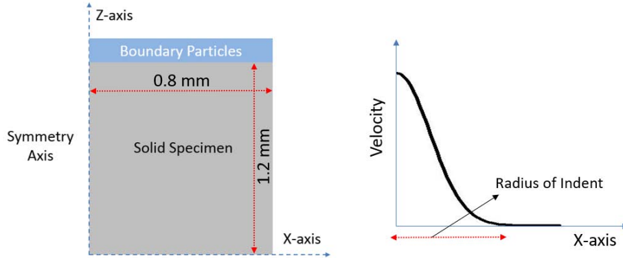
Figure 3. The figure on the left show the computational domain for solid simulation, the boundary particles marked in blue are given a downward velocity plotted on the right. (a Gaussian distribution is provided as the indent velocity as shown on the right, the radius of indent is defined as the distance from the center where the velocity is 1% of the peak value, a constant velocity is given to the indenter wrt time)
