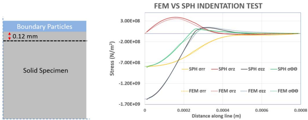
Figure 4. FEM results are compared against SPH for indentation of 6 microns in depth and 0.4 mm in radius for a stainless steel A-2205 specimen, the plots on right are plotted on the horizontal black dotted line (0.12 mm below the top surface) shown on the domain on the left.
