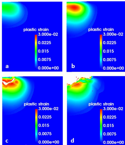
Figure 5. Sequence of images from damage simulation of a stainless steel A-2205 specimen, (a) Shows the plastic strain accumulation in material without damage, (b) high plastic strain zone just beneath the top surface, (c) damage initiation from the point of highest plastic strain, (d) material loss due to a single indent (domain size shown in the figure is same as in figure 3)
