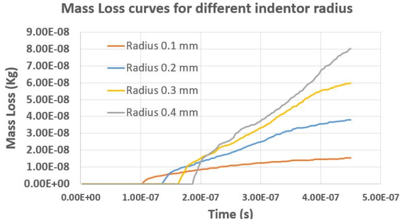
Figure 6. Mass loss curves for different indenter radius on a stainless steel A-2205 specimen obtained from SPH simulation, indentation depth is kept constant at 6 microns for all cases while the indenter radius is varied from 0.1 mm to 0.4 mm.
