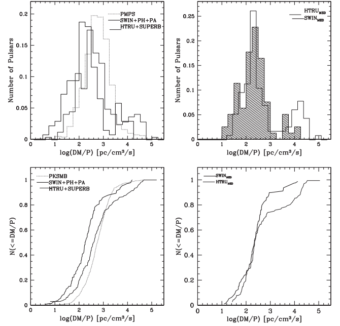
Figure 9. Normalized histograms (top) and cumulative distributions (bottom) of \text{DM}/P for Parkes survey discoveries. Left: the dotted curve is for the Galactic plane multibeam survey PMPS (Manchester et al. 2001), with a 3-MHz frequency resolution and a 250 \mu\text{s} time resolution; the solid thin curve is for surveys with the same frequency resolution, but 2\times finer time resolution (SWIN, Edwards et al. 2001; Jacoby et al. 2009; PH, Burgay et al. 2006; and PA, Burgay et al. 2013); the solid thick curve is for the most recent surveys using the BPSR digital backend, with 0.39-MHz frequency resolution and 64 \mu\text{s} time resolution (HTRU, Keith et al. 2010 and SUPERB, Keane et al. 2018). Right: comparison of intermediate-latitude Parkes surveys only. The shaded histogram is for the SWIN MED surveys, the thick solid line for HTRU-med.
