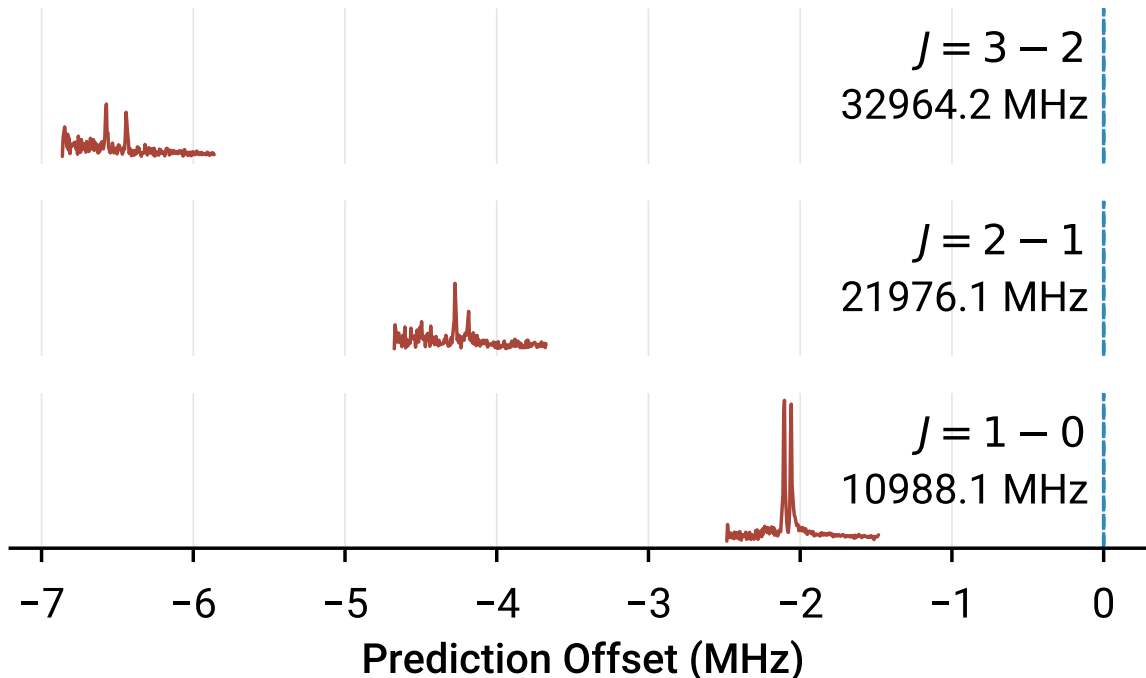
Figure 3: Illustration of the searches conducted for the lowest, a -type transitions of HCCSH. The blue lines indicate the ab initio predictions based on a harmonic J'(B_e + C_e) approximation, and the red traces show transitions observed consistently offset from the ab initio prediction. The doublet structure of the lines is due Doppler splitting, and arises from the co-linear configuration of the cavity axis with respect to that of the supersonic expansion.
