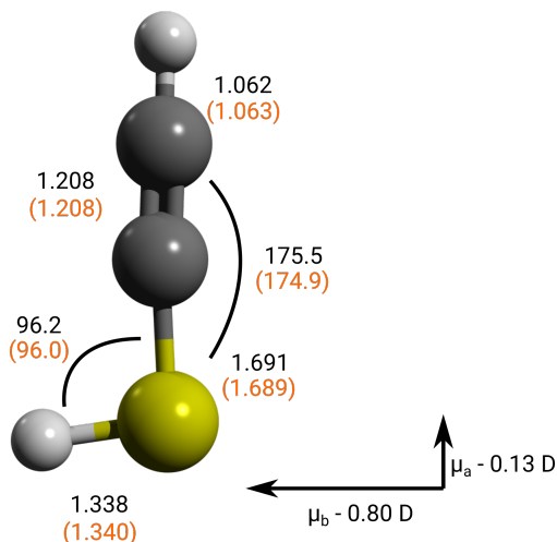
Figure 2: Equilibrium structure of HCCSH computed at the ae-CCSD(T) level of theory. Bond lengths are given in Å, angles in degrees. Values in black (without the parentheses) are obtained with core-valence basis functions (cc-pCVQZ), while the orange parameters correspond to the best-fit semi-experimental parameters (Table 4). Dipole moments (in Debye) are calculated using the CCSD(T)/cc-pCVQZ structure at the same level of theory.
