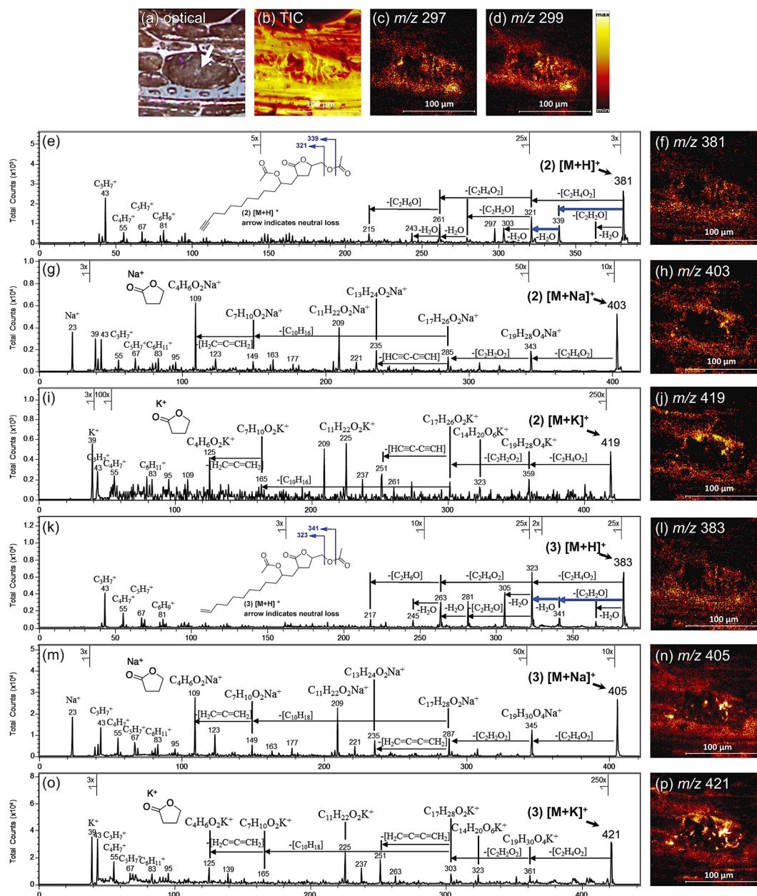
Figure 2. TOF-SIMS tandem MS imaging and product ion peak attributions. (a) Optical image of sapwood surface. (b) MS 1 total ion (TIC) image. MS 1 images of m/z 297 ions \gamma -lactone 4 rubrynlidide (c) and m/z 299 ions \gamma -lactone 5 rubrenolidide (d) were shown to give a comparison with the cellular localization of \gamma -lactones 2 and 3. (f) MS 2 TIC image of m/z 381 precursor ion. The product ion attributions shown in panel (e), MS/MS spectrum of the [M + H] + precursor ion at m/z 381, support the structure of \gamma -lactone 2. (h) MS 2 TIC image of m/z 403 precursor ion. The product ion attributions shown in panel (g), MS/MS spectrum of the [M + Na] + precursor ion at m/z 403, support the structure of \gamma -lactone 2. (j) MS 2 TIC image of m/z 419 precursor ion. The product ion attributions shown in panel (i), MS/MS spectrum of [M + K] + precursor ion at m/z 419, support the structure of \gamma -lactone 2. (l) MS 2 TIC image of m/z 383 precursor ion. The product ion attributions shown in panel (k), MS/MS spectrum of the [M + H] + precursor ion at m/z 383, support the structure of \gamma -lactone 3. (n) MS 2 TIC image of m/z 405 precursor ion. The product ion attributions shown in panel (m), MS/MS spectrum of the [M + Na] + precursor ion at m/z 405, support the structure of \gamma -lactone 3. (p) MS 2 TIC image of m/z 421 precursor ion. The product ion attributions shown in panel (o), MS/MS spectrum of [M + K] + precursor ion at m/z 421, support the structure of \gamma -lactone 3. Each ion image has a field-of-view of 150 \mu m x 150 \mu m with a pixel dimension of 586 nm. In panels e and k the characteristic neutral losses are indicated, while in panels g–j, m–p the alkali metal adducts of oxolan-2-one are shown at m/z 109 and m/z 125.
