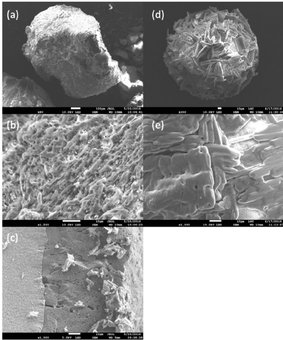
Fig. 13. SEM images of SF particles impregnated by WI at 0.44 \text{ g}^{\text{H}_2\text{O}}/\text{g}^{\text{Support}} : (a) full particle, (b) external surface, and (c) cross-section of the particle. SEM images of SS particles impregnated by WI at 0.36 \text{ g}^{\text{H}_2\text{O}}/\text{g}^{\text{Support}} : (d) full particle and (e) external surface.
