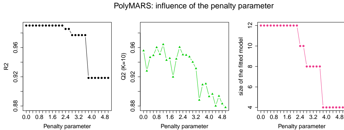
Figure 24: Study of the influence of the penalty parameter on the performance of a PolyMARS model fitted on the learning set. The plot represents the R2 computed on the training set (left-hand side), the evolution of Q2 estimated using 10-folds cross validation (middle) and the number of terms (right-hand side).
