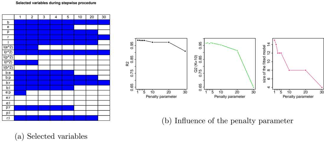
Figure 23: The impact of the penalty parameter on the stepwise procedure. (a) variables included (rows = variables, columns = penalty) and (b) quality criteria.
