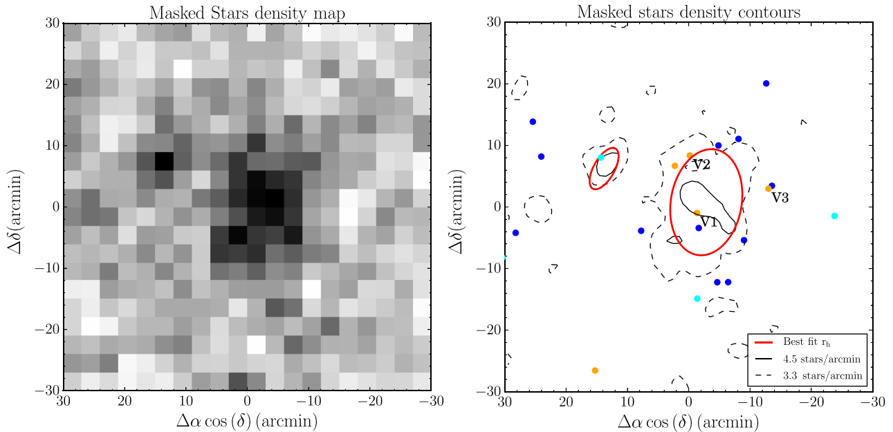
Figure 4. Deep follow-up imaging of the Carina satellites Left: Density map of stars within a CMD mask defined by the best-fitting isochrone of Carina II. Right: Density contours of the same region of the sky with the half-light radius of the best-fitting models overplotted in red. Stars within 0.3 mag from the BHB ridge line of Car II(III) are shown in blue(cyan), and RR Lyrae stars found in the field are shown in orange. Both overdensities are clearly seen in the density maps and are well reproduced by the models.
