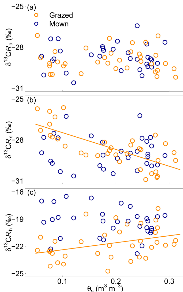
Figure 4. ^{13}\text{C} isotopic signature of \text{CO}_2 respired from the roots and rhizosphere ( \delta^{13}\text{C}_{\text{ra}} , panel a), the whole soil ( \delta^{13}\text{C}_{\text{rs}} , panel b) and the root- and rhizosphere-free soil ( \delta^{13}\text{C}_{\text{rh}} , panel c) as functions of soil volumetric water content ( \theta_s ) for the grazed (orange circles) and mown (blue circles) grasslands. The lines represent the fit of linear regressions. Only significant correlations appear.
