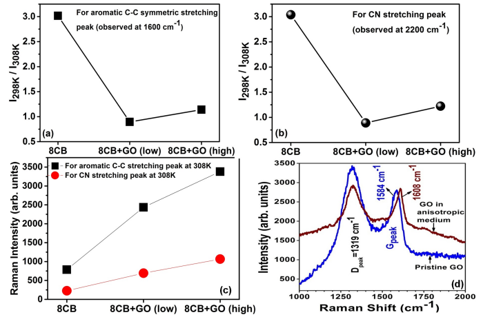
Fig. 4 The variation of intensity ratio ( I_{298K}/I_{308K} ) as a function of temperature for (a) aromatic C-C symmetric stretching at \approx 1600\text{ cm}^{-1} and (b) CN stretching at \approx 2200\text{ cm}^{-1} for 8CB LC and 8CB+GO hybrid material having low (wt % \leq 0.2 ) and high (wt % > 0.2 ) dispersion concentration of GO flakes. (c) shows the change in Raman intensity of aromatic C-C stretching and CN stretching peaks at 308 K whereas (d) shows the Raman spectra of GO in pristine form and in the anisotropic (8CB) medium.
