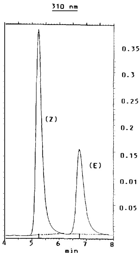
Fig. 1. HPLC separation of an artificial mixture of ( Z )- and ( E )-dodecyl urocanate isomers. Column, \mu Porasil ( 10\ \mu\text{m} ) ( 30\ \text{cm} \times 4\ \text{mm} I.D.); detection, absorption at 310\ \text{nm} ; mobile phase, chloroform-ethanol (85:15); flow-rate, 0.7\ \text{ml/min} ; temperature = 20^\circ\text{C} ; injection: 15\ \mu\text{l} of an approximately 10^{-3}\ \text{mol l}^{-1} solution. Values on the y -axis are absorbance units.
