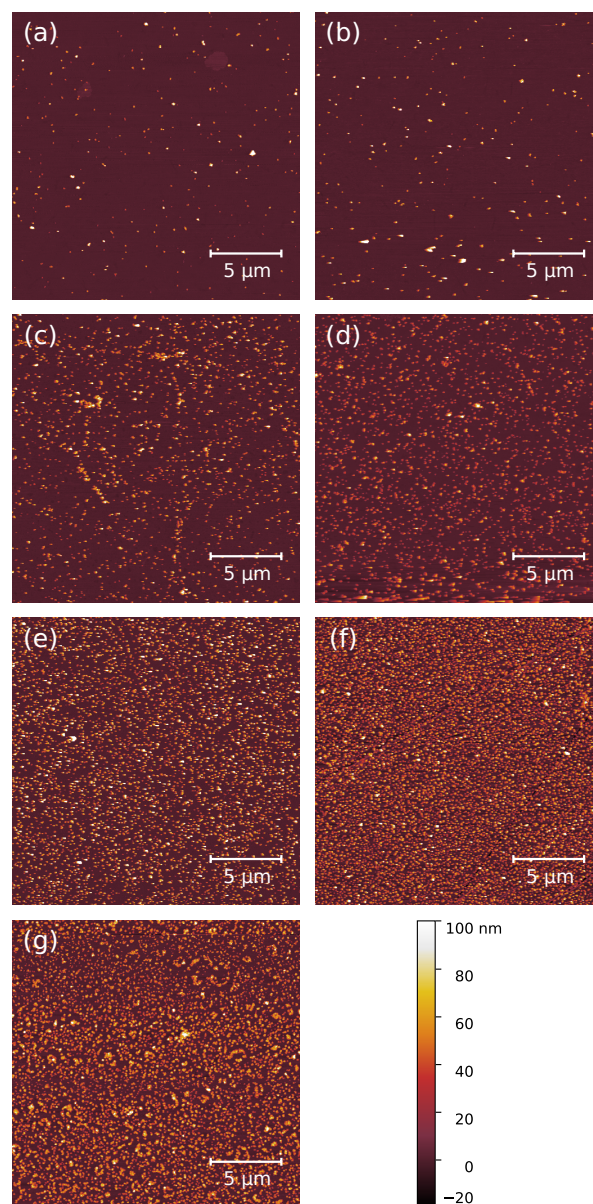
Fig. 2 AFM images with scale bar 20 x 20 \mu\text{m} of the PBA NPs deposited on the amino-gold surface with different initial concentrations: (a) 0.04 mg.mL -1 ; (b) 0.08 mg.mL -1 ; (c) 0.16 mg.mL -1 ; (d) 0.31 mg.mL -1 ; (e) 0.62 mg.mL -1 ; (f) 1.50 mg.mL -1 ; (g) 2.50 mg.mL -1 .
