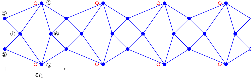
Figure 6. Slightly asymmetrical pantographic beam. Nodes 4 and 5 have been slightly moved on the right from their previous positions (here in red) of Figure 3.
