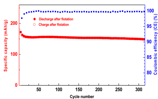
Fig. 10. Cycling stability of natural graphite (Raw and concentrate graphite) vs. Na.
