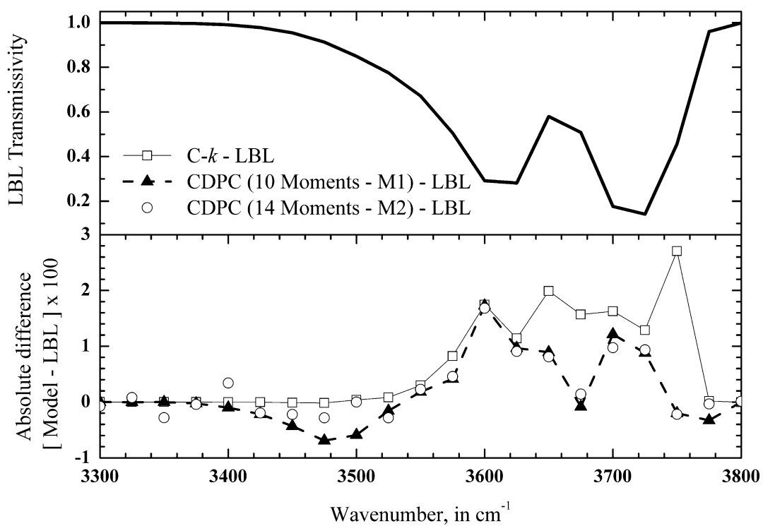
Figure 6. Narrow band ( 25 \text{ cm}^{-1} ) transmission function for a non-uniform path (see text for details) – Top: LBL reference calculation. Bottom: absolute difference \times 10^2 between LBL and approximate models (C- k , CDPC with methods M1 and M2).
