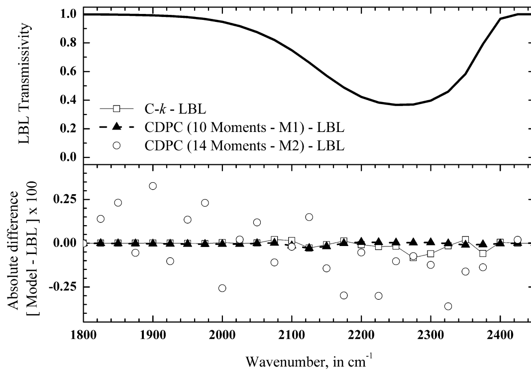
Figure 3. Narrow band ( 25 \text{ cm}^{-1} ) transmission function for 10 cm of 10 % \text{CO}_2 – 90 % \text{N}_2 at 2900 K and 1 atmosphere – Top: LBL reference calculation. Bottom: absolute difference \times 10^2 between LBL and approximate models (C- k , CDPC with methods M1 and M2).
