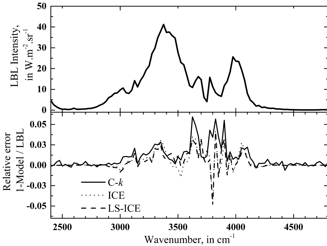
Figure 10. Case C6. Narrow band intensity for a non-uniform \text{H}_2\text{O} - \text{N}_2 mixture (see text for details) calculated by the LBL, C- k and \ell -distribution models with two non-uniform approximations (ICE and LS-ICE).
