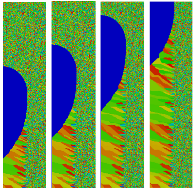
Fig. 9 Orientation of cells at different time steps for a cellular automaton simulation based on J210 thermal simulation and a KGT2 growth kinetic model
